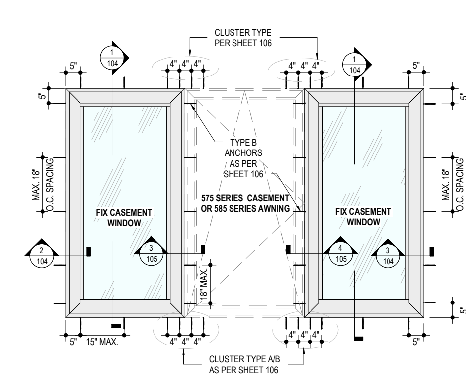
6 102 ALTERNATIVE ELEVATION 4 NOT TO SCALE
