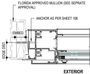
4 106 ANCHORAGE INTO ALUMINUM MULLION NOT TO SCALE
