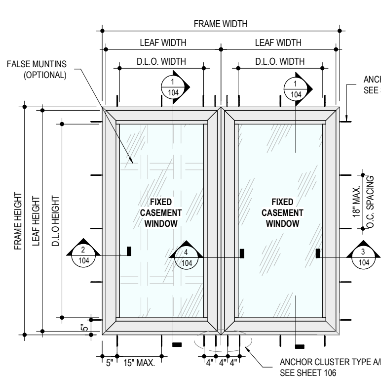
1 102 TYPICAL FIX CASEMENT ELEVATION NOT TO SCALE
