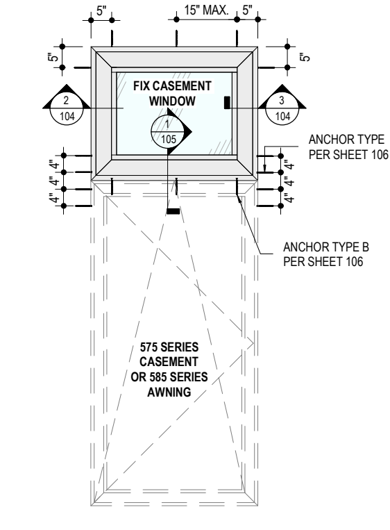
4 102 ALTERNATIVE ELEVATION 1 NOT TO SCALE
