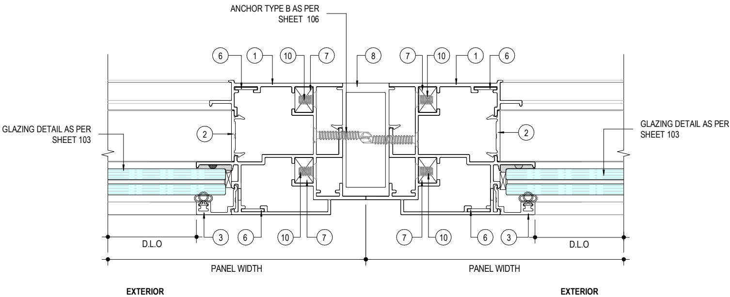
2 104 FIX CASEMENT JAMB DETAIL 1 NOT TO SCALE
