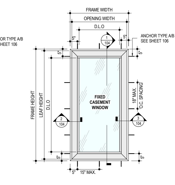
2 102 TYPICAL SINGLE FIX CASEMENT ELEVATION NOT TO SCALE
