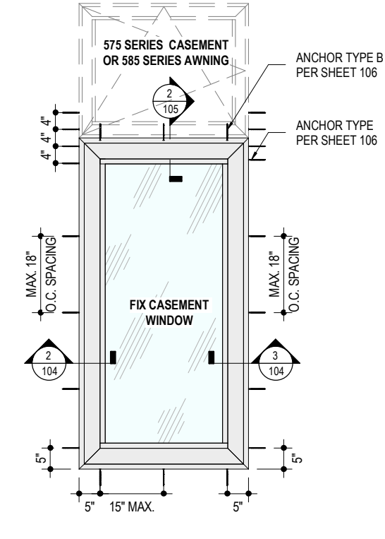
3 102 ALTERNATIVE ELEVATION 2 NOT TO SCALE
