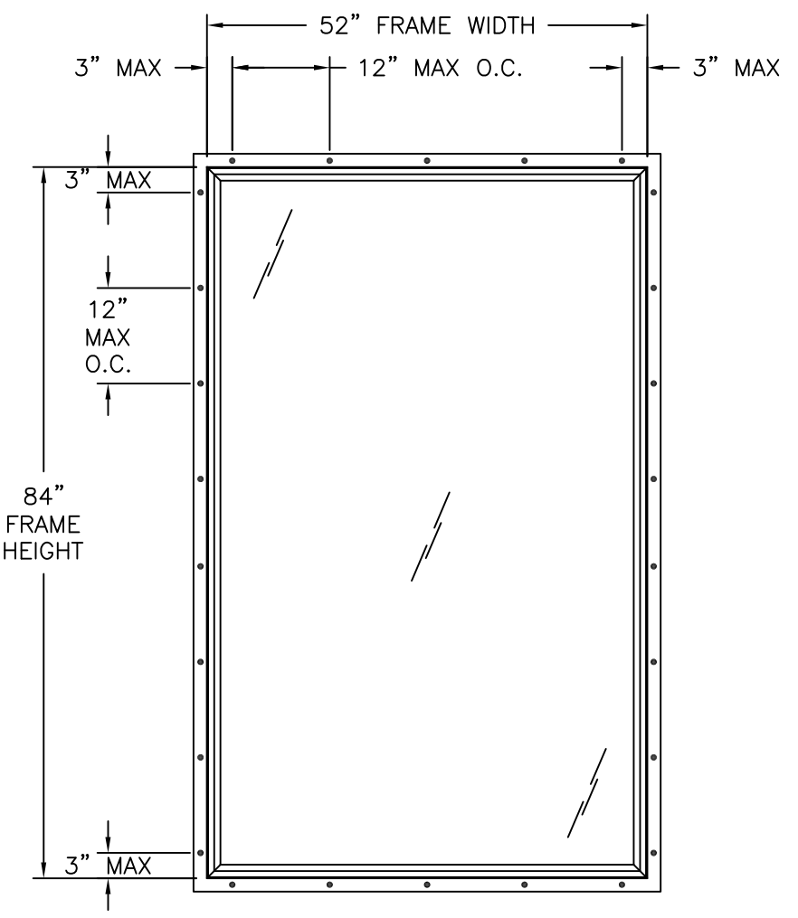
G250 PVC FIXED WINDOW FIN INSTALLATION
