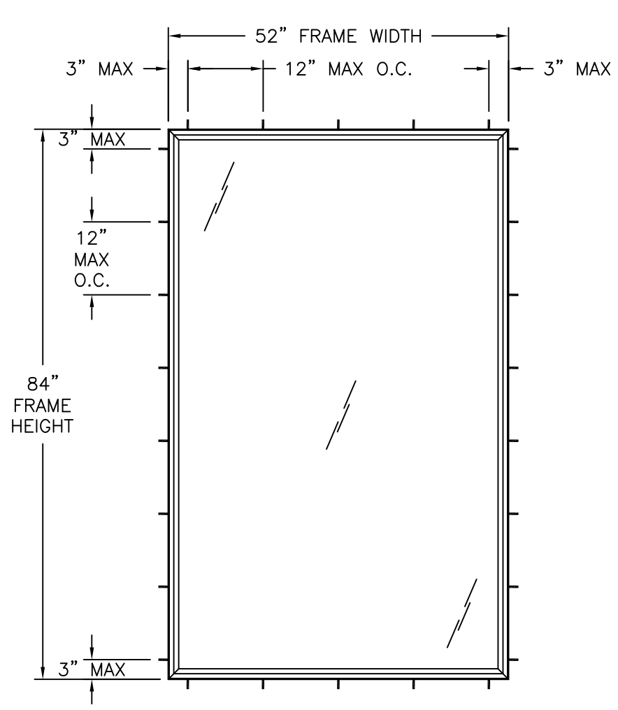
G250 PVC FIXED WINDOW FINLESS, FLANGE AND STRAP INSTALLATION
