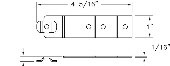
STRAP 18GA STEEL
