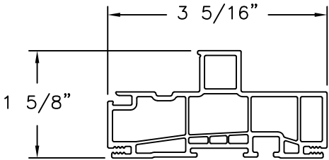
MAIN FRAME (1841A) EXTRUDED PVC
