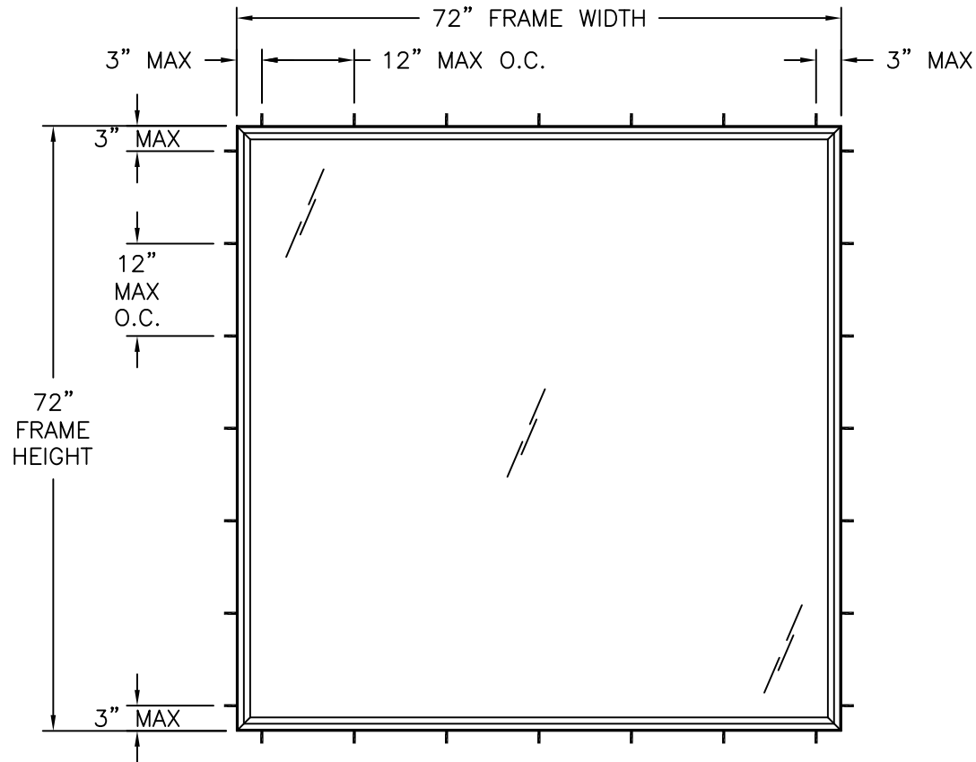
G250 PVC FIXED WINDOW FINLESS, FLANGE AND STRAP INSTALLATION
