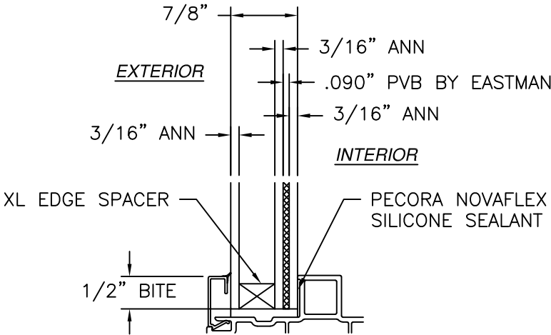
GLAZING DETAIL
