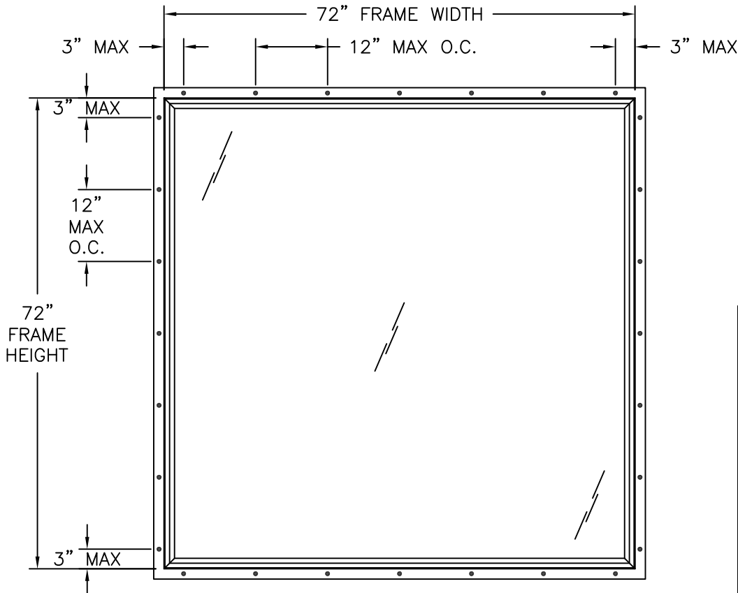
G250 PVC FIXED WINDOW FIN INSTALLATION
