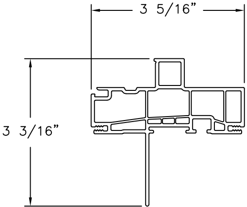
MAIN FRAME (1861AJ) EXTRUDED PVC
