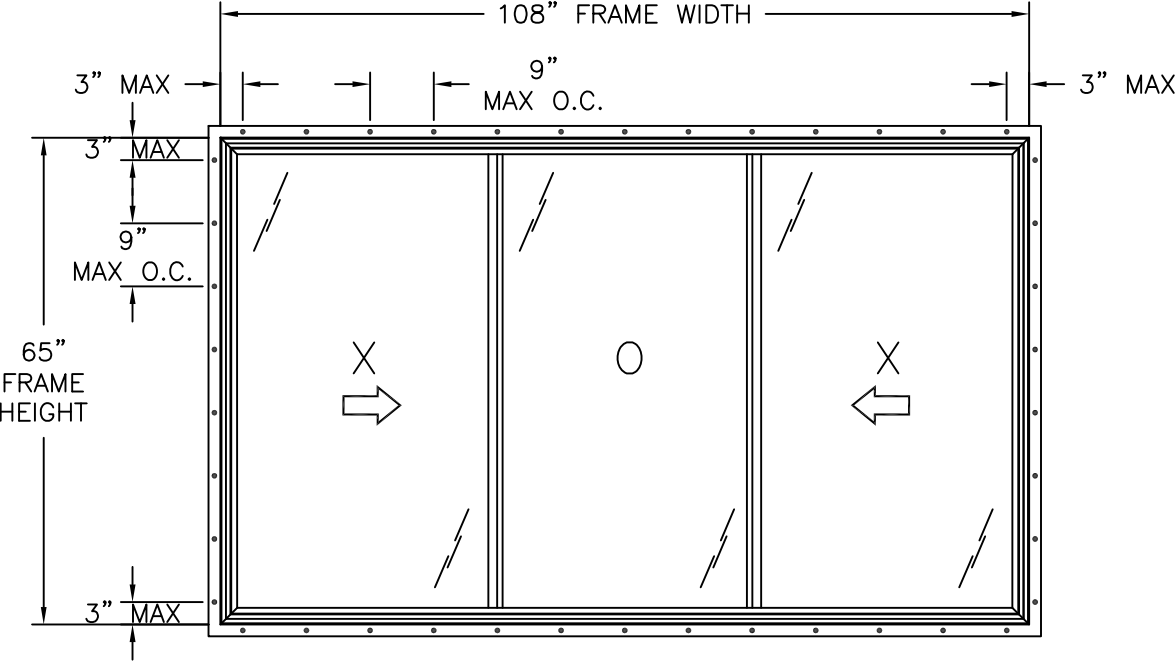
G140 PVC HORIZONTAL SLIDER WINDOW FIN INSTALLATION
