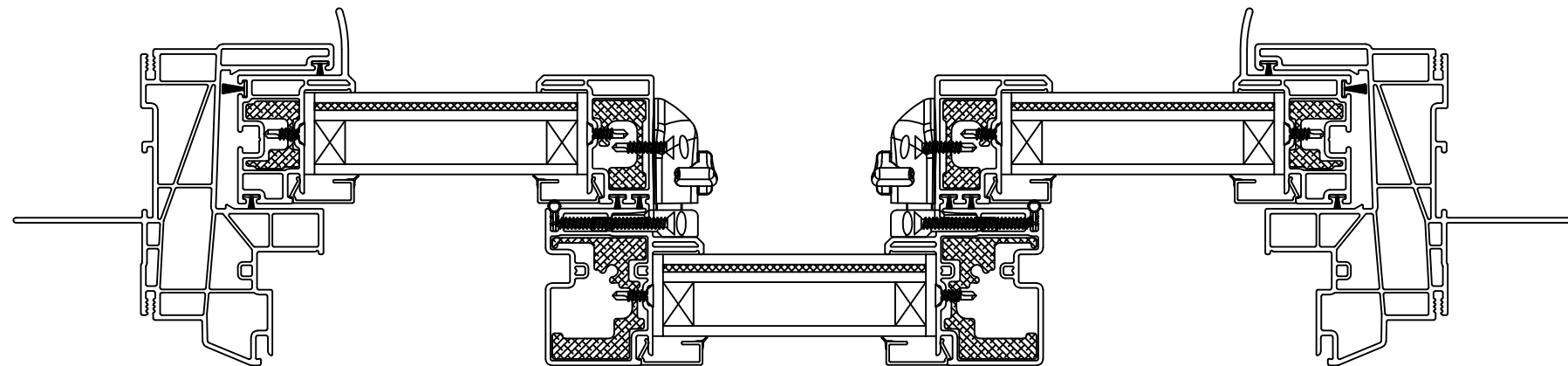
HORIZONTAL CROSS SECTION FIN INSTALLATION
