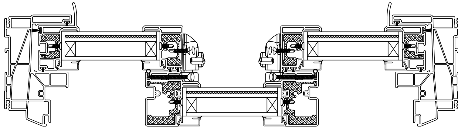
HORIZONTAL CROSS SECTION FINLESS INSTALLATION
