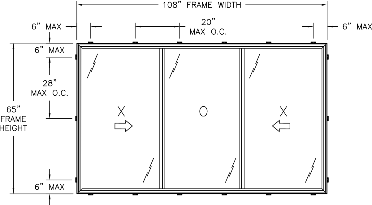
G140 PVC HORIZONTAL SLIDER WINDOW STRAP INSTALLATION
