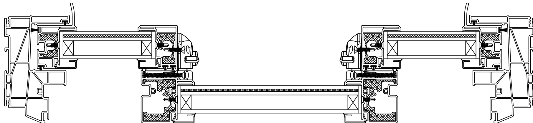
HORIZONTAL CROSS SECTION FINLESS INSTALLATION
