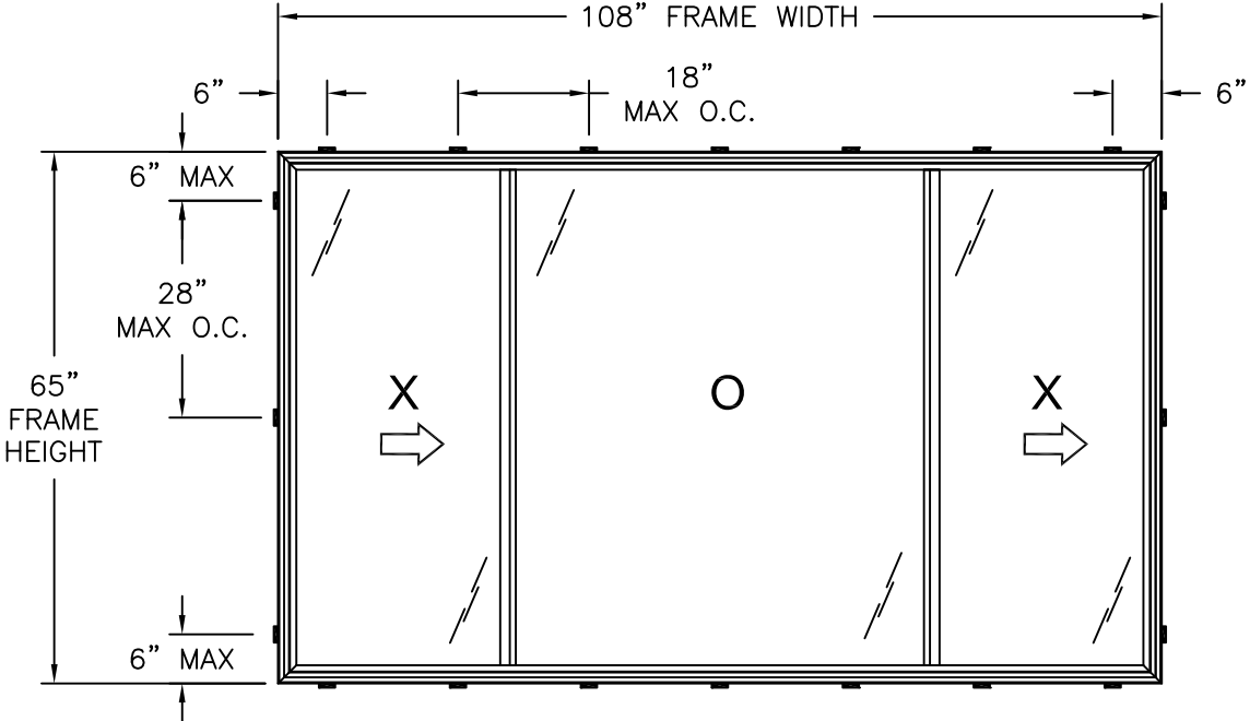
G140 PVC HORIZONTAL SLIDER WINDOW STRAP INSTALLATION
