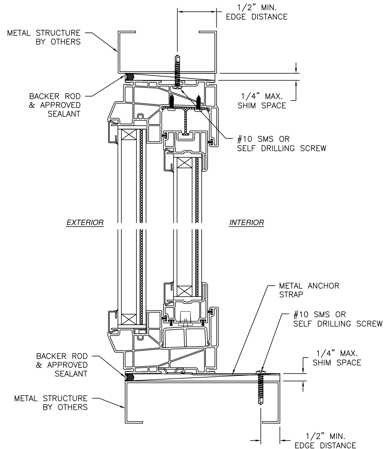
VERTICAL CROSS SECTION METAL STRUCTURE INSTALLATION
