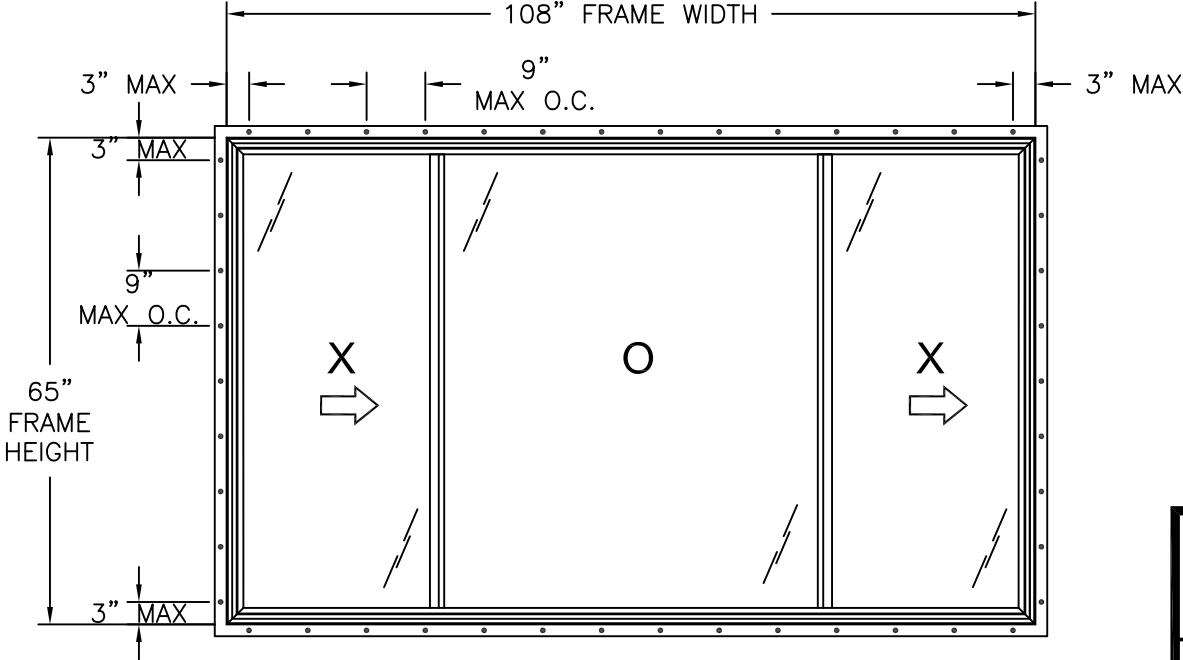
G140 PVC HORIZONTAL SLIDER WINDOW FIN INSTALLATION
