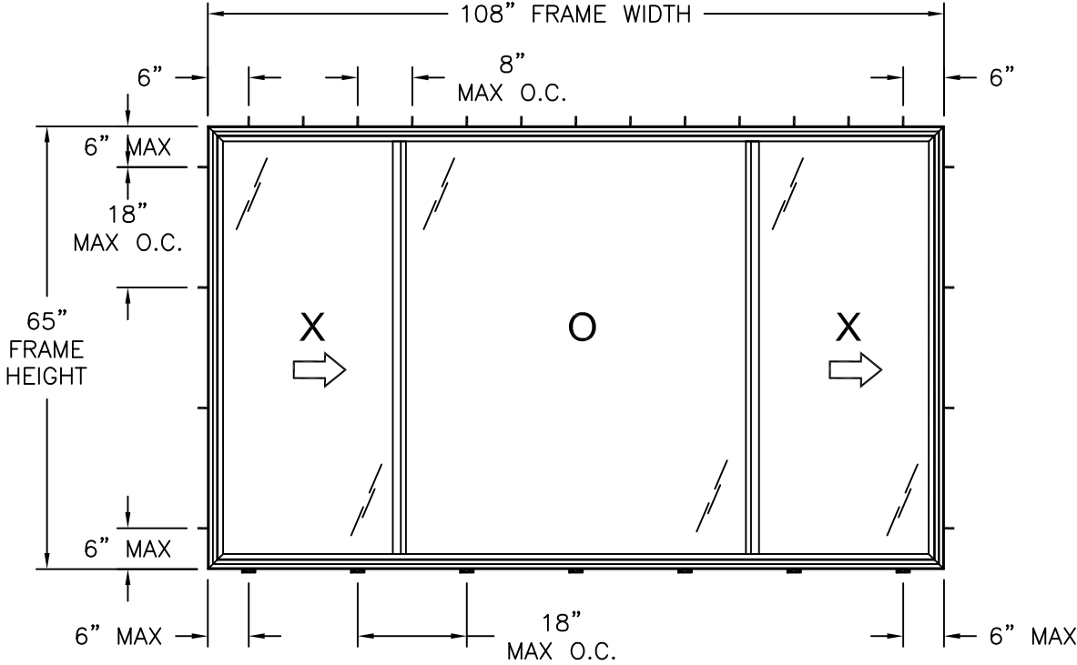
G140 PVC HORIZONTAL SLIDER WINDOW FINLESS AND FLANGE INSTALLATION
