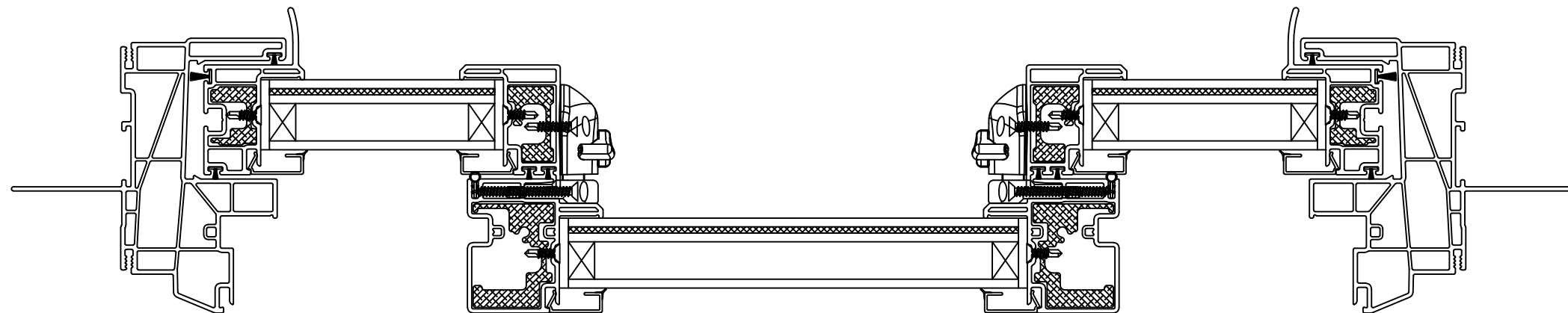
HORIZONTAL CROSS SECTION FIN INSTALLATION
