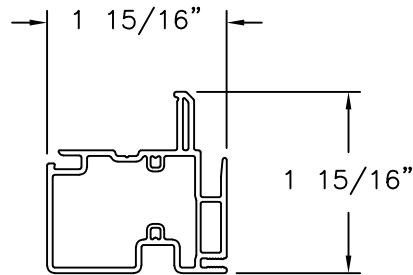
FIXED MEETING STILE (1837) EXTRUDED PVC
