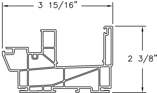
MAIN FRAME (1834) EXTRUDED PVC
