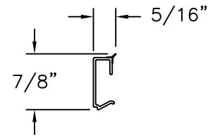
GLAZING BEAD (836B) EXTRUDED PVC
