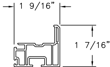
TOP RAIL (1879) EXTRUDED PVC
