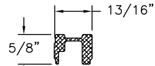
REINFORCEMENT (16579) ALUMINUM 6063-T5
