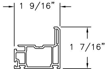
BOTTOM RAIL (1808) EXTRUDED PVC
