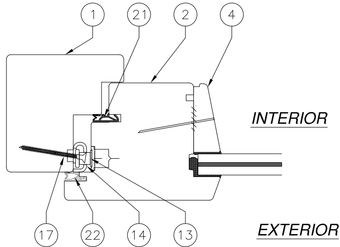
HORIZONTAL CROSS SECTION W/ CONCEALED HINGE
