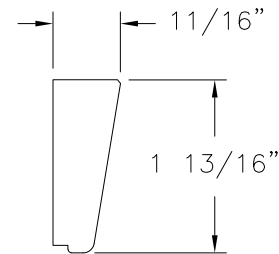
④ GLASS STOP WOOD SPECIFIC GRAVITY G.59 MIN.
