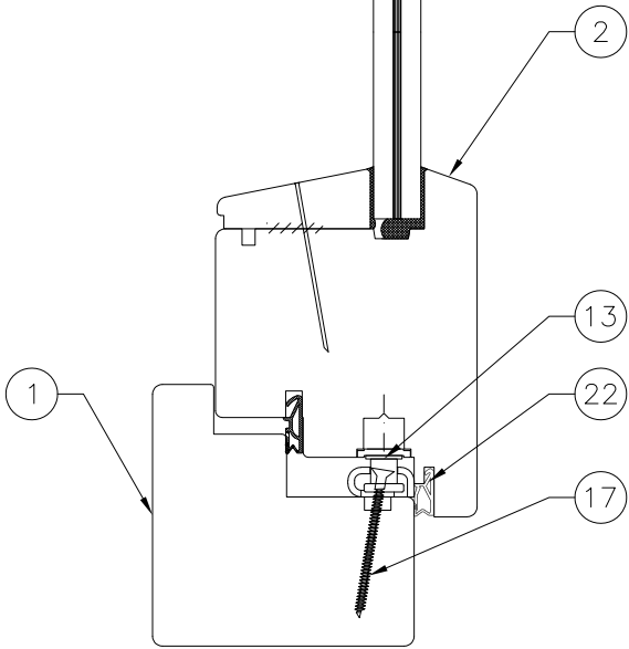
VERTICAL SECTION
