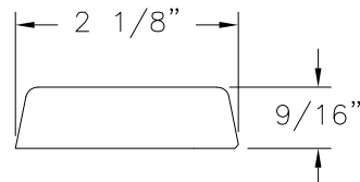
⑥ FLAST ASTRAGAL WOOD SPECIFIC GRAVITY G.59 MIN.
