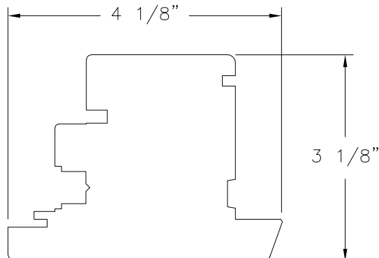
② SASH WOOD SPECIFIC GRAVITY G.59 MIN.
