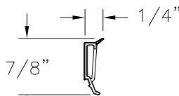
GLAZING BEAD (10005470) EXTRUDED VINYL
