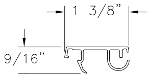
SASH STOP (10008483) ALUMINUM 6005-T5
