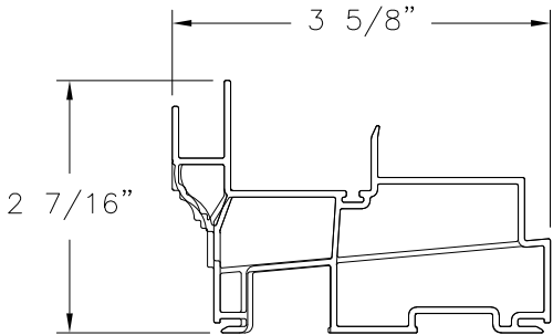
HEAD FINLESS (10008652) EXTRUDED VINYL
