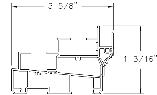
JAMB FINLESS (10008654) EXTRUDED VINYL
