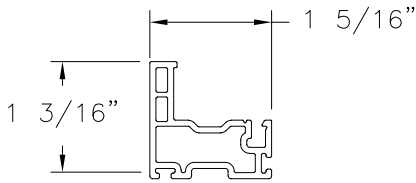
MAIN SASH (10008875) EXTRUDED VINYL
