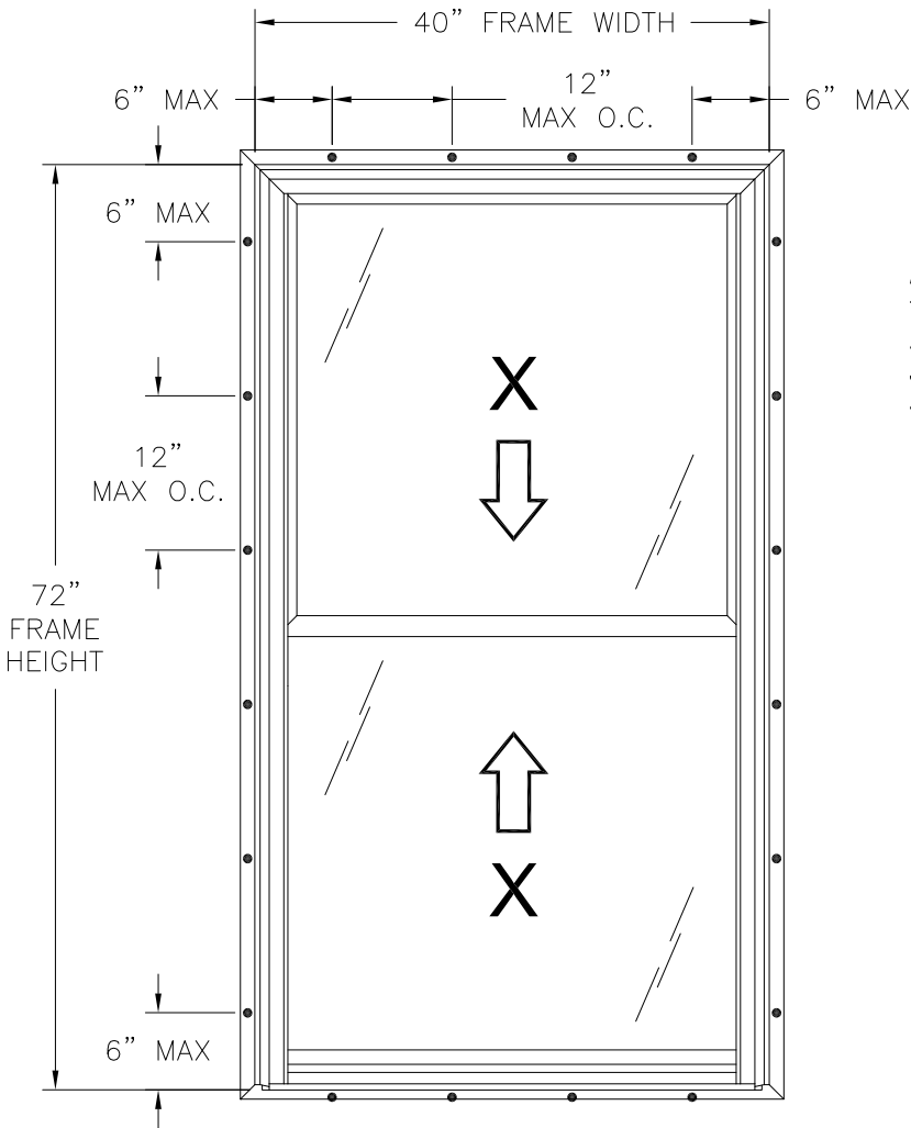
ACADIAN COMPASS SERIES DOUBLE HUNG WINDOW EXTERIOR VIEW FINLESS INSTALLATION
