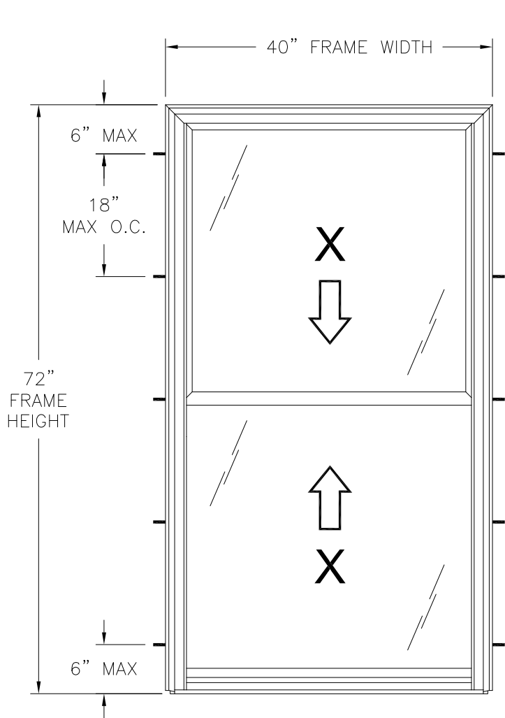
ACADIAN COMPASS SERIES DOUBLE HUNG WINDOW EXTERIOR VIEW FINLESS INSTALLATION
