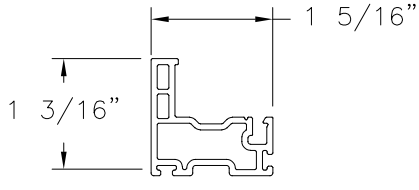
MAIN SASH (10008875) EXTRUDED VINYL
