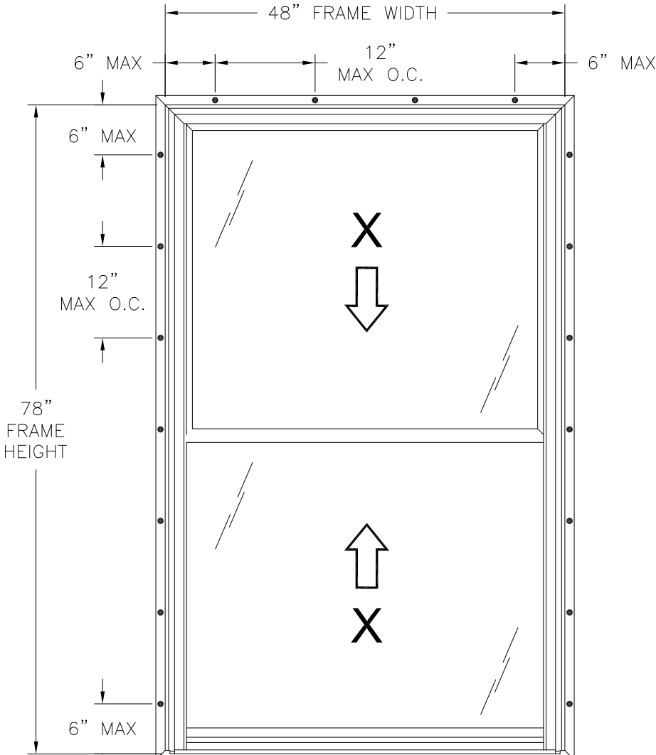
ACADIAN COMPASS SERIES DOUBLE HUNG WINDOW EXTERIOR VIEW FINLESS INSTALLATION
