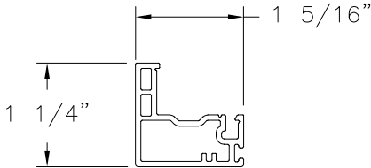
LOCK RAIL (10008885) EXTRUDED VINYL
