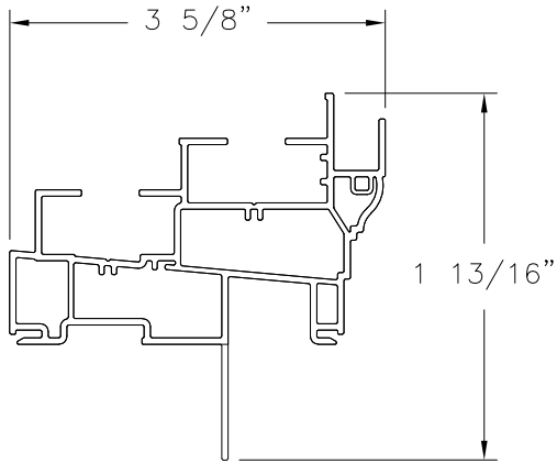
JAMB FIN (10008653) EXTRUDED VINYL
