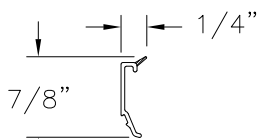
GLAZING BEAD EXTRUDED VINYL
