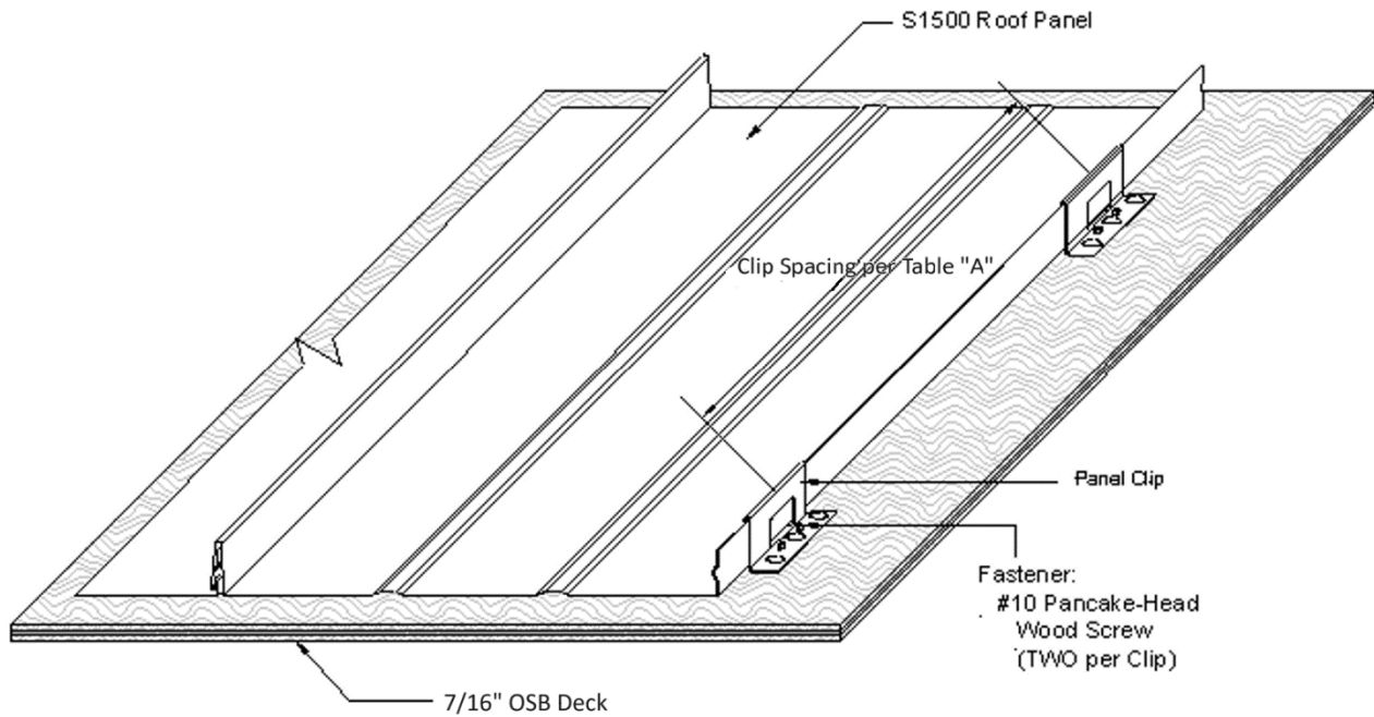
Typical Roof Assembly Isometric View
