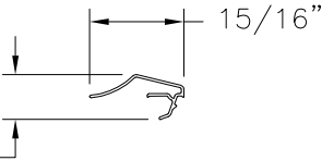
SCREEN RETAINER (10005258) EXTRUDED RIGID PVC
