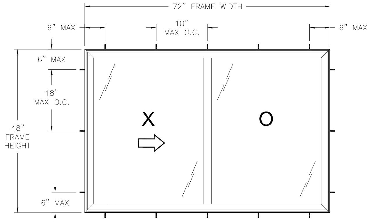
ACADIAN COMPASS SERIES SINGLE SLIDER FINLESS INSTALLATION EXTERIOR VIEW
