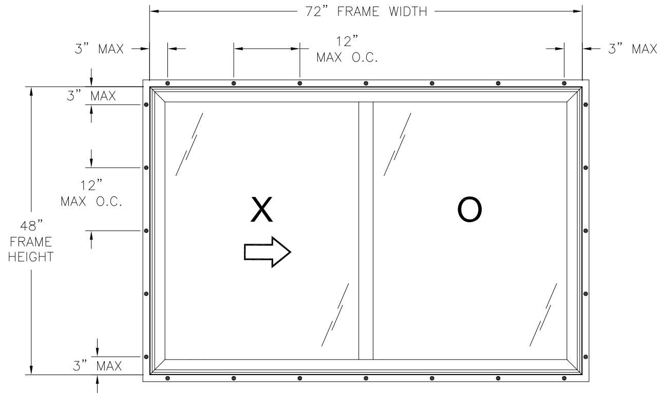
ACADIAN COMPASS SERIES SINGLE SLIDER FIN INSTALLATION EXTERIOR VIEW
