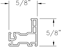
MAIN SASH (10008875) VINYL PVC
