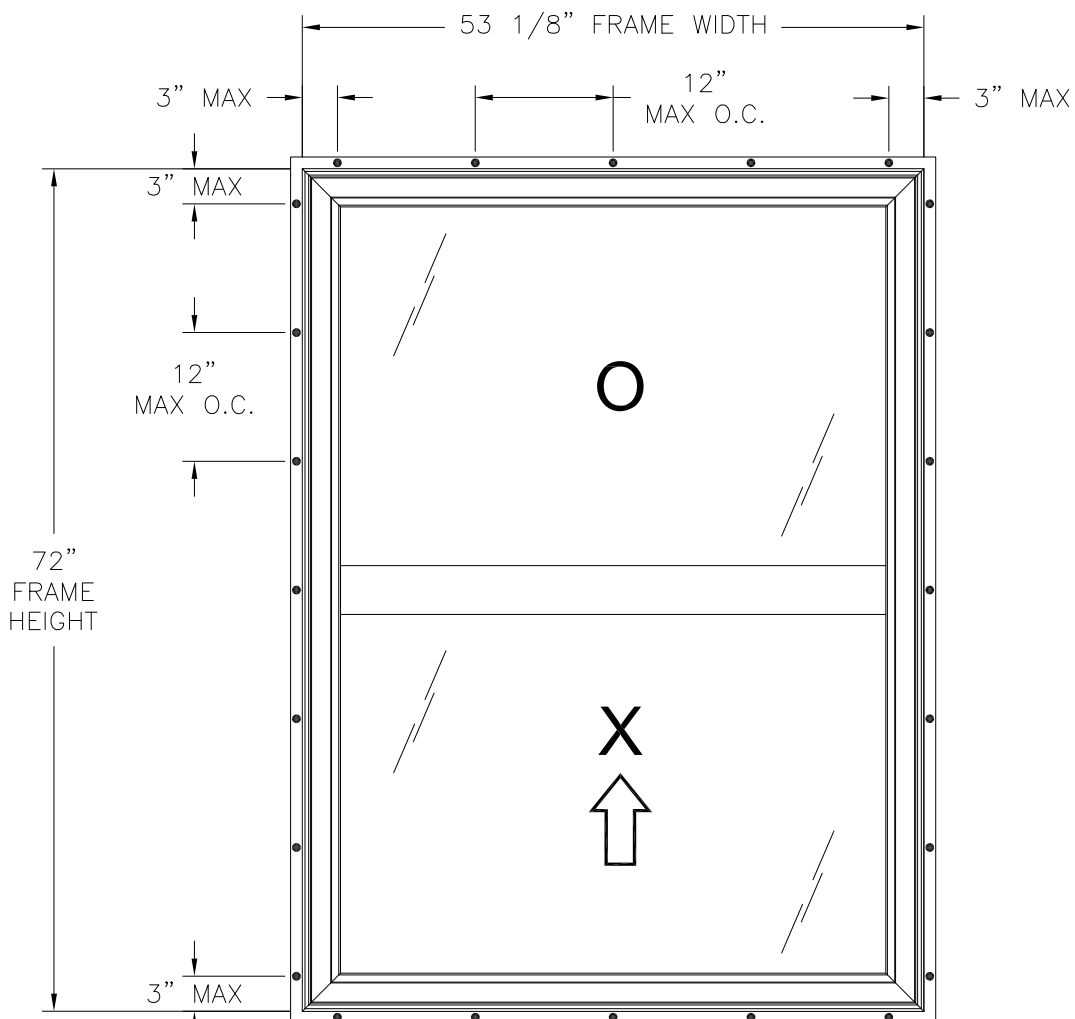
ACADIAN WINDOWS IMPACT SERIES SINGLE HUNG EXTERIOR VIEW FIN INSTALLATION
