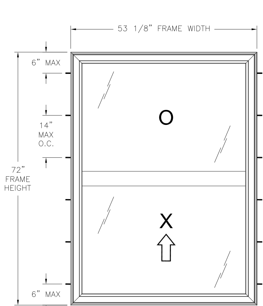
ACADIAN WINDOWS IMPACT SERIES SINGLE HUNG EXTERIOR VIEW FINLESS INSTALLATION
