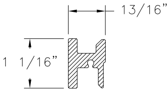
REINFORCEMENT (10000670) DNA PUR
