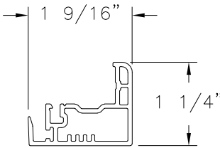
LOCK SASH (10008845) RIGID PVC
