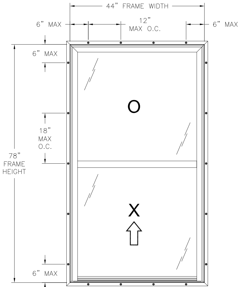
ACADIAN COMPASS SERIES SINGLE HUNG EXTERIOR VIEW FIN INSTALLATION
