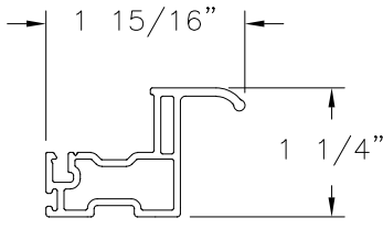
PULL/LIFT SASH (10008882) RIGID PVC
