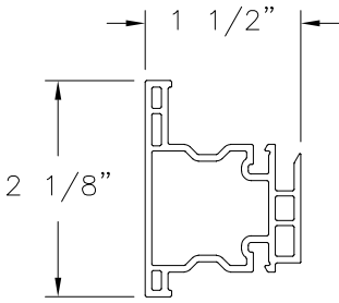
MEETING RAIL (10008511) RIGID PVC
