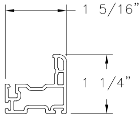
MAIN SASH (10008842) RIGID PVC
