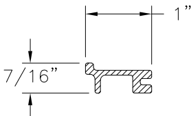
REINFORCEMENT (10000661) DNA PUR
