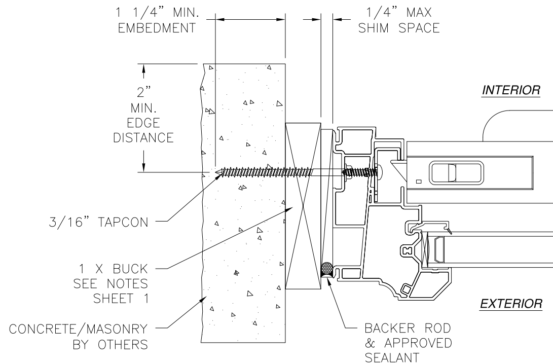
JAMB INSTALLATION DETAIL CONCRETE/MASONRY INSTALLATION
