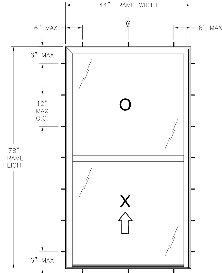
ACADIAN COMPASS SERIES SINGLE HUNG EXTERIOR VIEW FINLESS INSTALLATION
