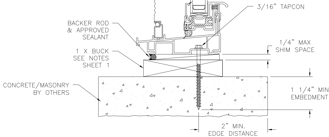
VERTICAL CROSS SECTION CONCRETE/MASONRY WITH INSTALLATION
