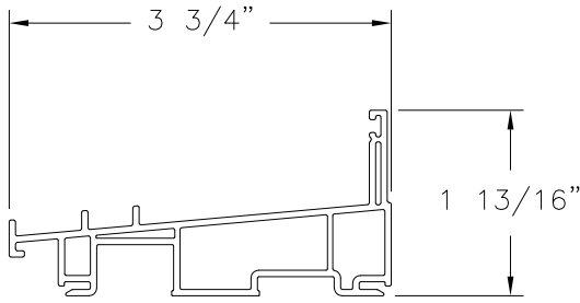
SILL FINLESS (10008673) RIGID PVC
