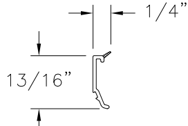
GLAZING BEAD (10008127) RIGID PVC
