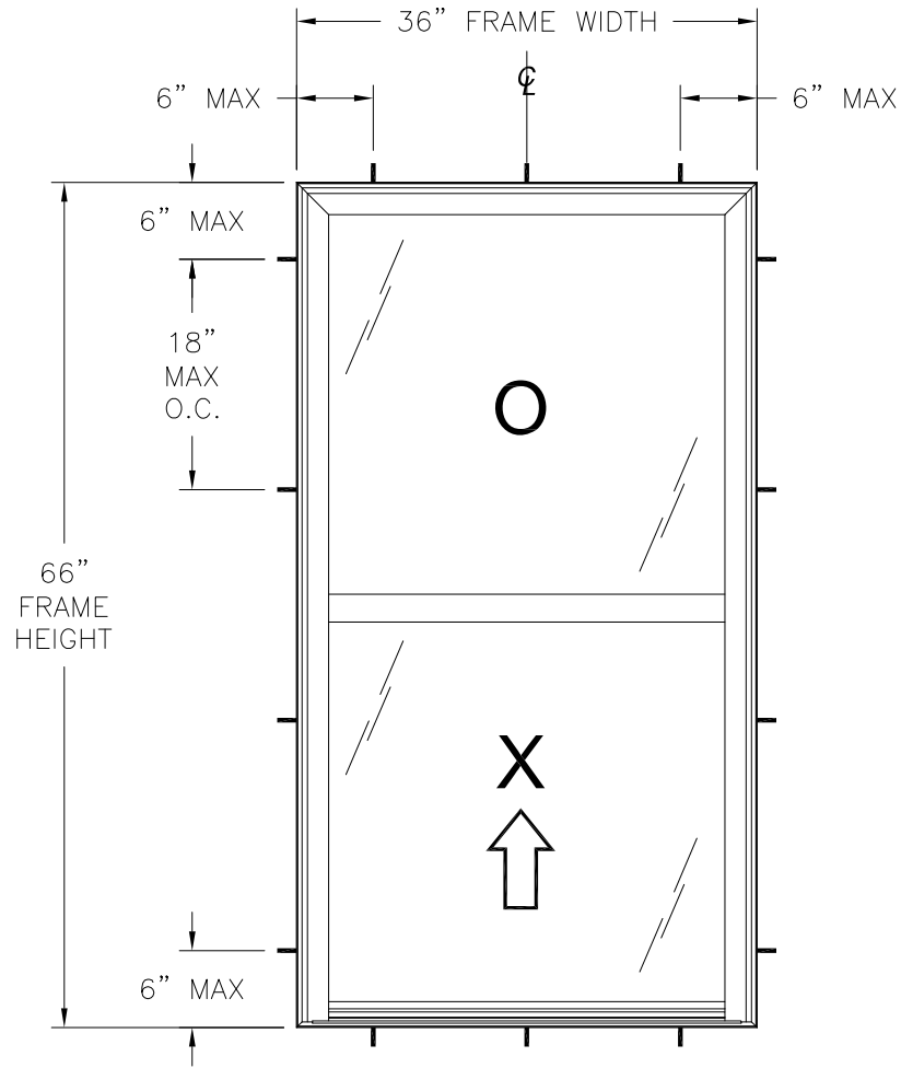
ACADIAN COMPASS SERIES SINGLE HUNG EXTERIOR VIEW FIN INSTALLATION
