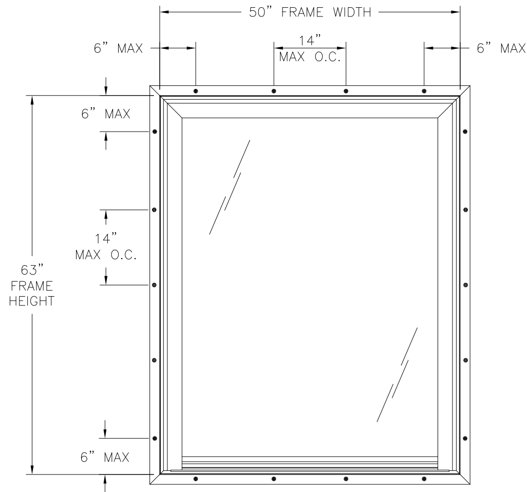
ACADIAN WINDOW IMPACT SERIES FIXED FIN INSTALLATION EXTERIOR VIEW
