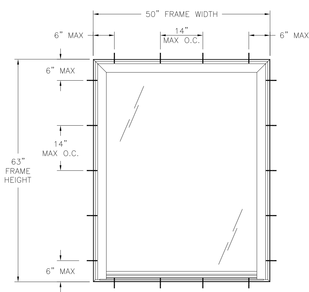
ACADIAN WINDOW IMPACT SERIES FIXED FRAME INSTALLATION EXTERIOR VIEW
