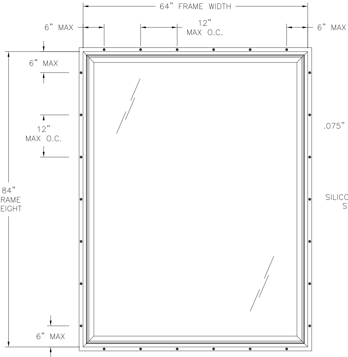
ACADIAN WINDOW IMPACT SERIES FIXED FIN INSTALLATION EXTERIOR VIEW
