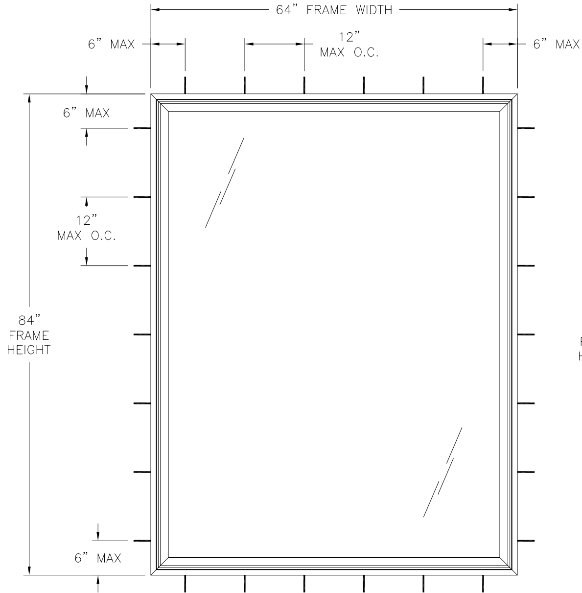
ACADIAN WINDOW IMPACT SERIES FIXED FRAME INSTALLATION EXTERIOR VIEW
