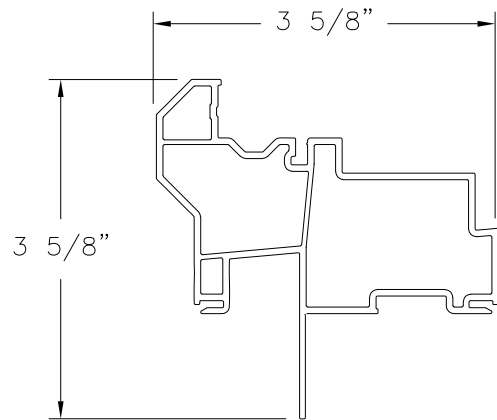
MAIN FRAME (10008676) FIN INSTALLATION RIGID PVC
