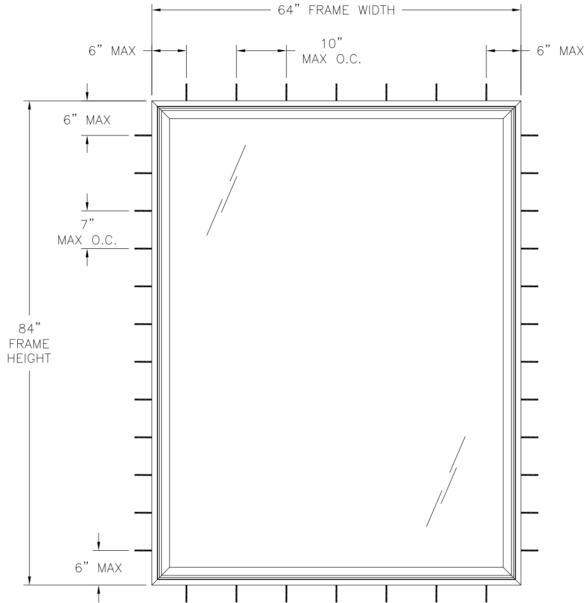
ACADIAN NON-IMPACT SERIES FIXED WINDOW FRAME INSTALLATION EXTERIOR VIEW
