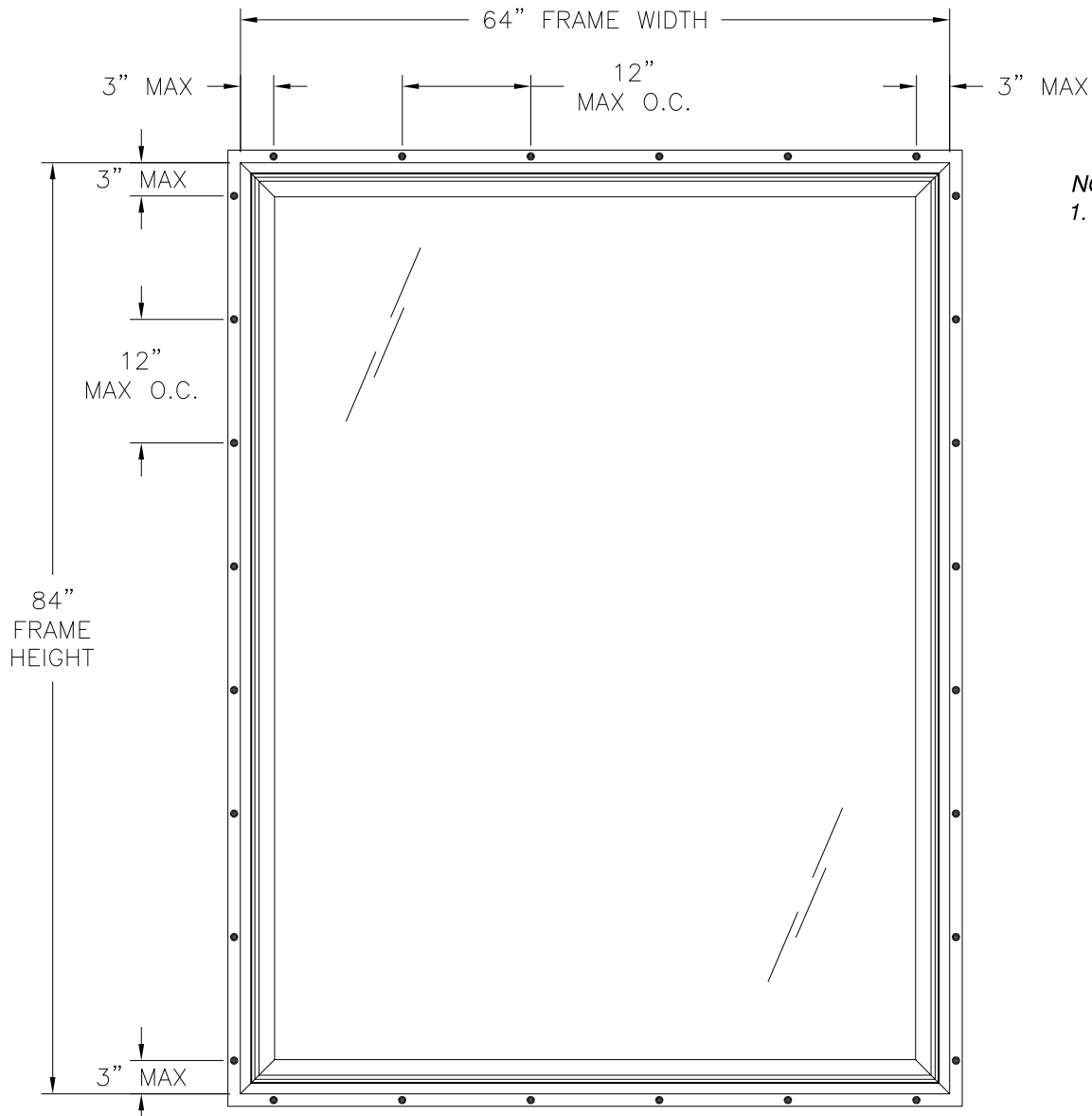
ACADIAN NON-IMPACT SERIES FIXED WINDOW FIN INSTALLATION EXTERIOR VIEW
