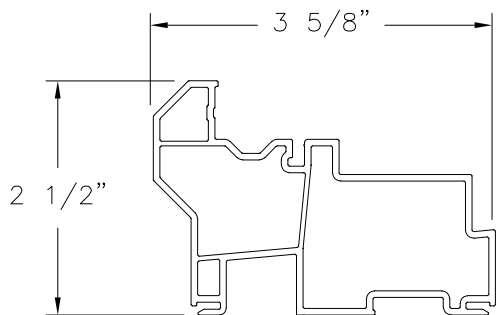
MAIN FRAME (10008696) FINLESS INSTALLATION RIGID PVC
