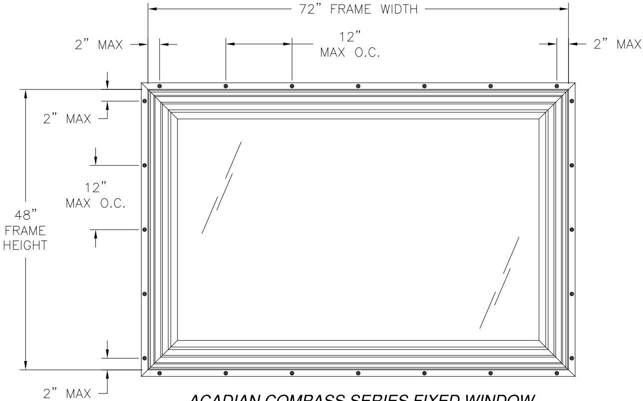
ACADIAN COMPASS SERIES FIXED WINDOW FIN INSTALLATION EXTERIOR VIEW
