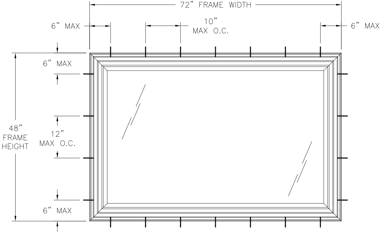
ACADIAN COMPASS SERIES FIXED WINDOW FRAME INSTALLATION EXTERIOR VIEW
