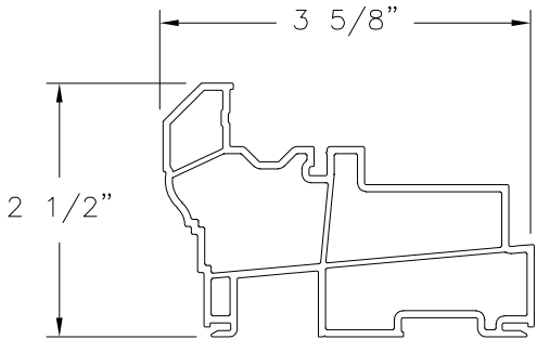
MAIN FRAME (10008656) FINLESS INSTALLATION RIGID PVC
