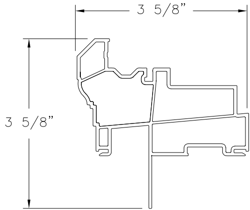
MAIN FRAME (10008656) FIN INSTALLATION RIGID PVC
