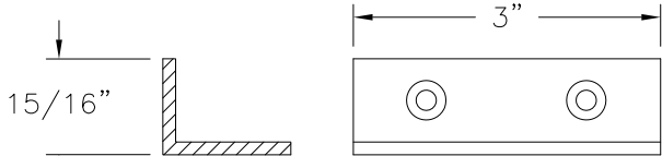
ANGLE ALUMINUM 6063-T5, 1/8" THICKNESS
