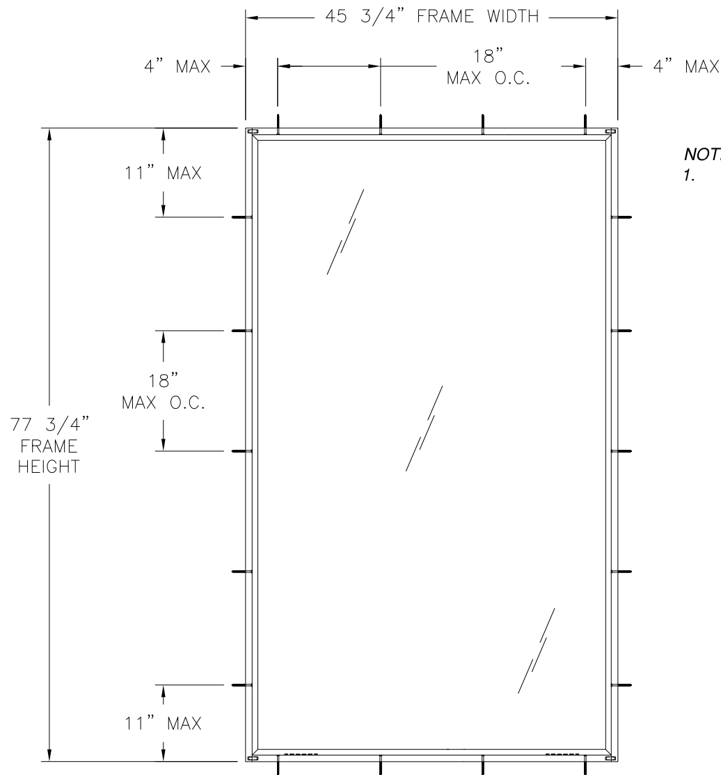
FIXED WINDOW AW60 EXTERIOR VIEW
