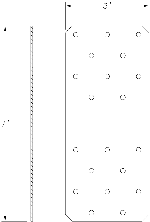
HTP37Z STRAP GALVANIZED STEEL, 16 GA
