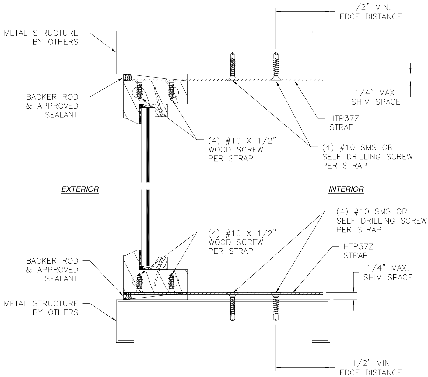
VERTICAL CROSS SECTION METAL STRUCTURE INSTALLATION
