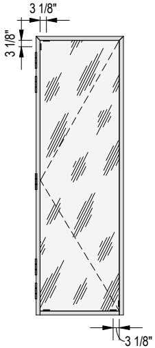
SETTING BLOCKS LAYOUT
