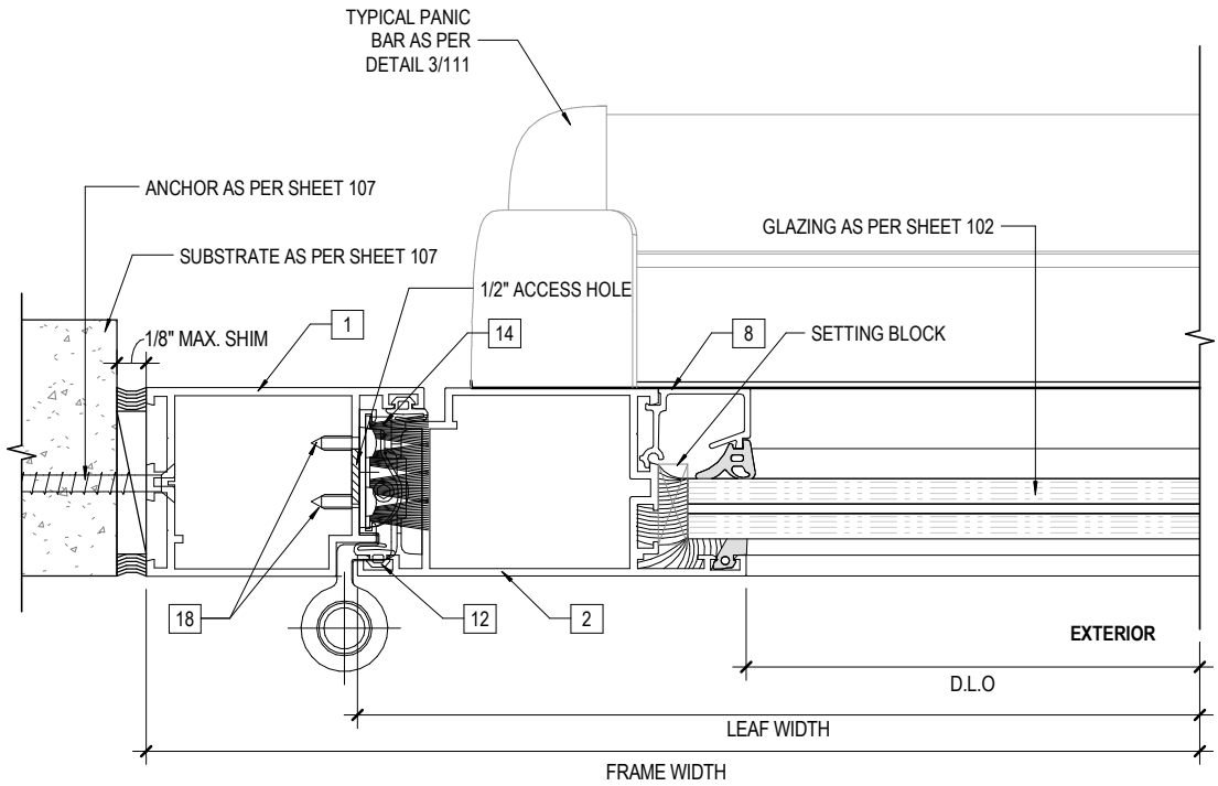
2 106 JAMB DETAIL WITH PANIC BAR N.T.S
