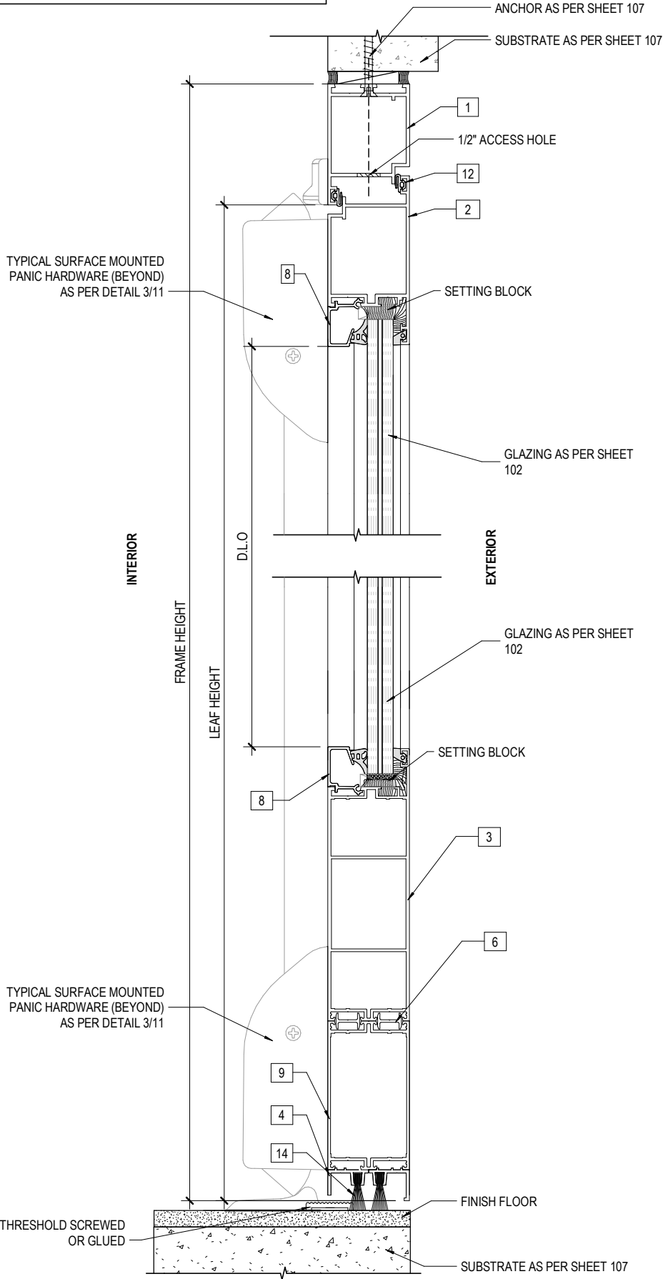
1 106 HEAD AND SILL DETAIL WITH PANIC BAR N.T.S
