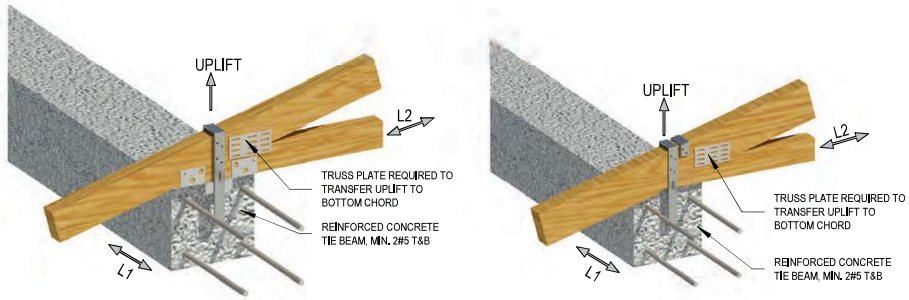
NVSTA 12H TO 44H INSTALLATION
