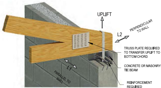
TYPICAL NVTH/NVTHS INSTALLATION
