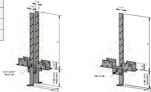
NVHTA WITH 14G DOUBLE NVTH STRAP
