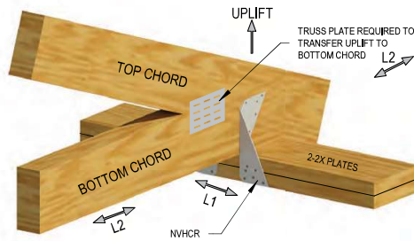
TYPICAL NVHCR/L INSTALLATION
