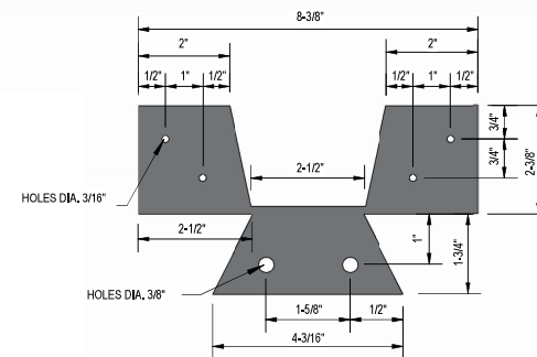
NV358 & NV458 18G SEAT DETAIL
