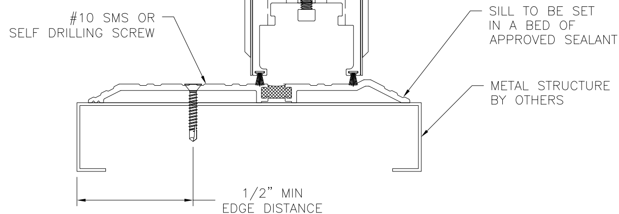
VERTICAL CROSS SECTION METAL STRUCTURE INSTALLATION
