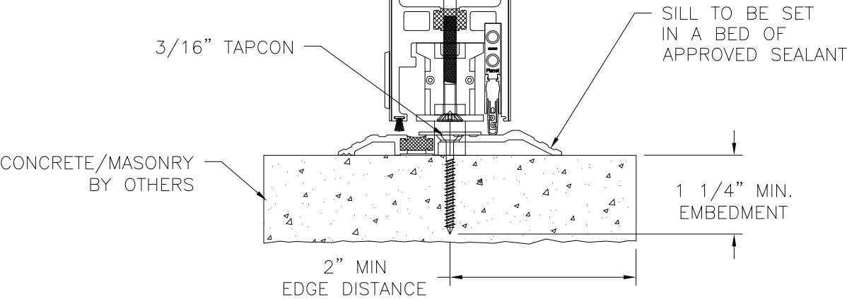
VERTICAL CROSS SECTION CONCRETE/MASONRY INSTALLATION
