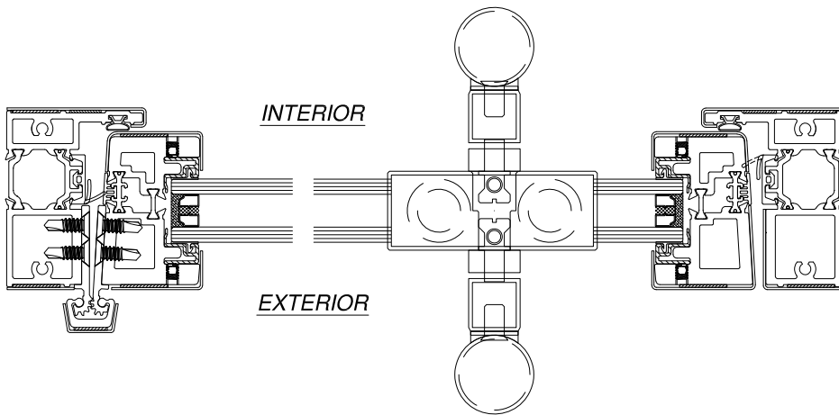
HORIZONTAL CROSS SECTION
