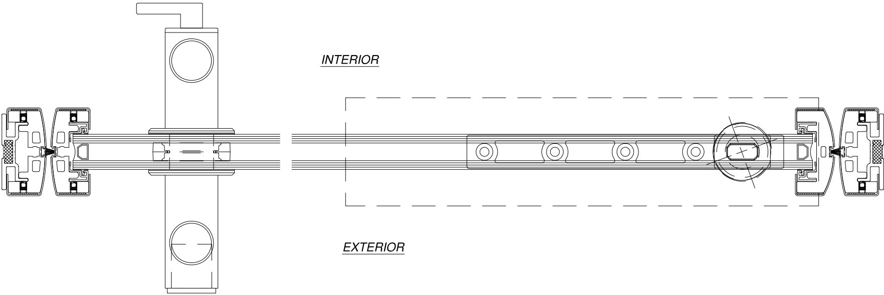
HORIZONTAL CROSS SECTION
