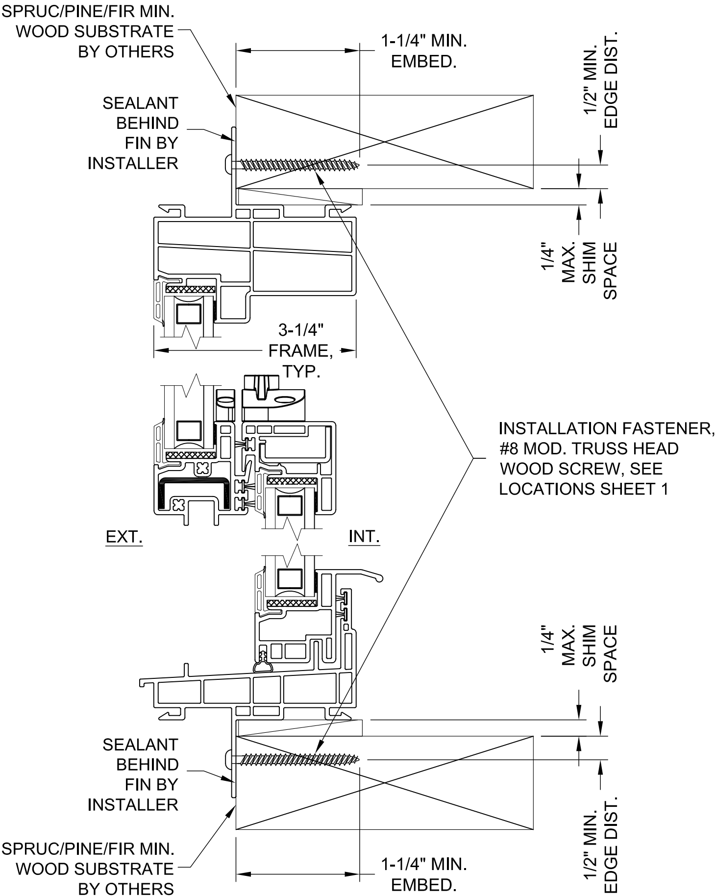
TYPICAL VERTICAL SECTION
