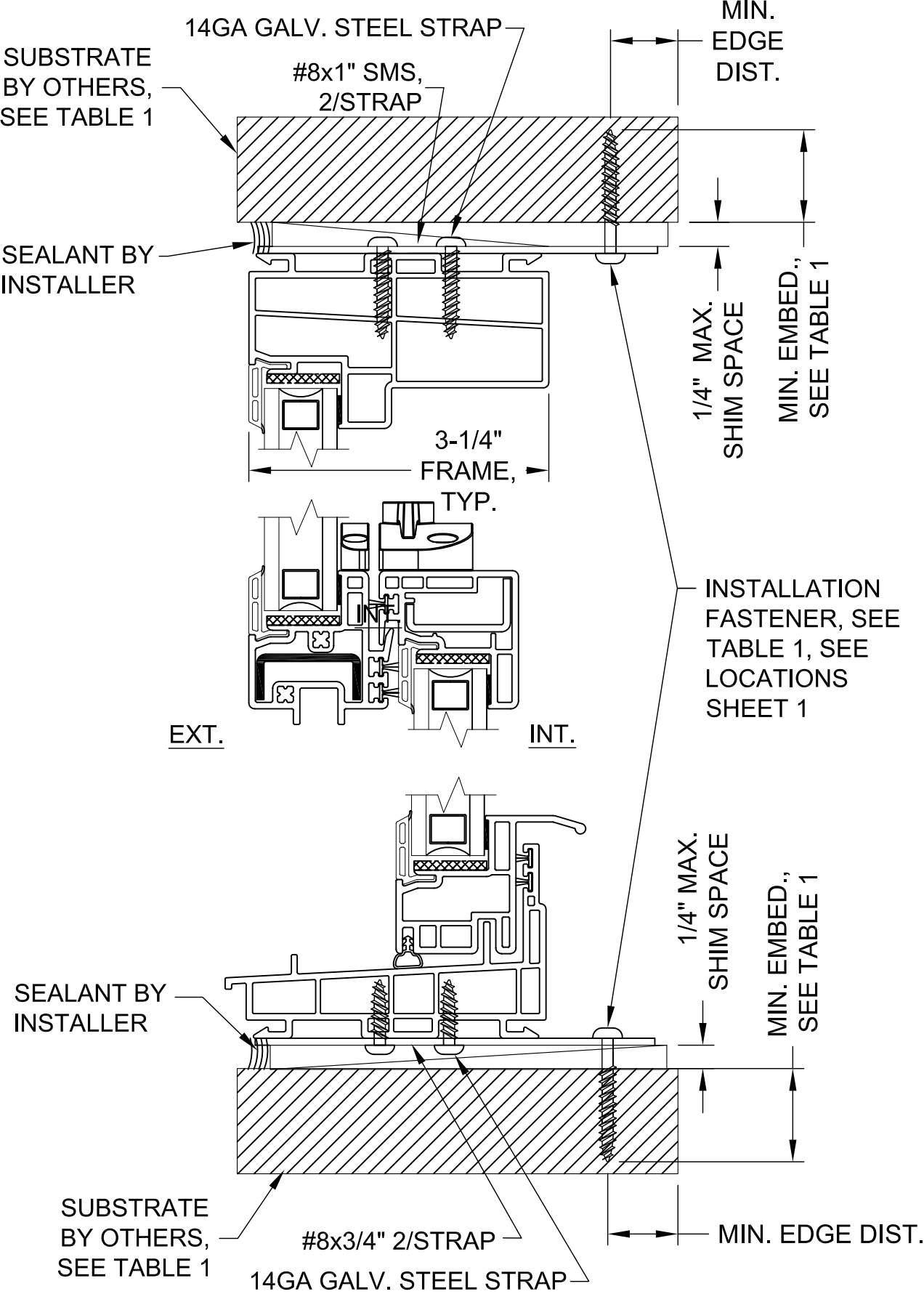
TYPICAL VERTICAL SECTION
