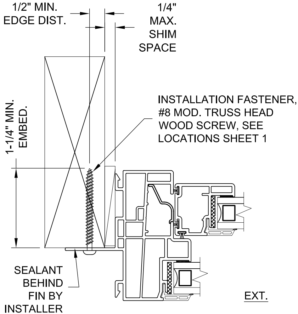
TYPICAL JAMB HORIZONTAL SECTION
