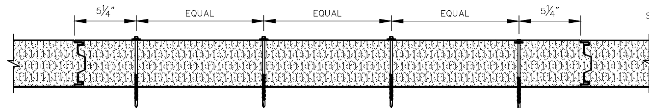
PANEL INSTALLATION SECTION AT INTERIOR SUPPORTS-TSFP2
