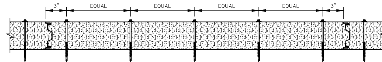
PANEL INSTALLATION SECTION AT END SUPPORTS-TSFPMAX
