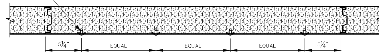
PANEL INSTALLATION SECTION AT INTERIOR SUPPORTS-TSFP3
