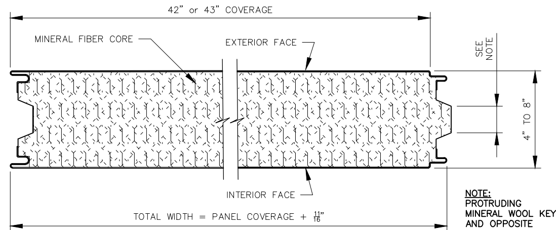
4-INCH THRU 8-INCH THERMSAFE PANEL
