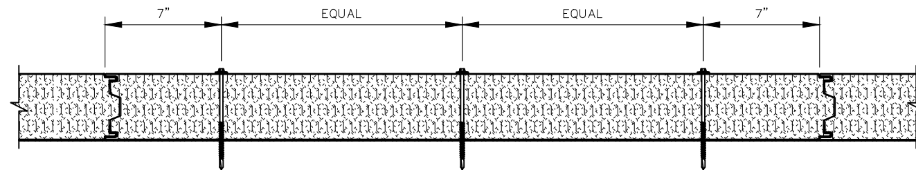
PANEL INSTALLATION SECTION AT INTERIOR SUPPORTS-TSFP1
