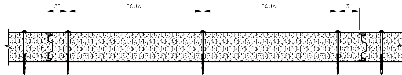
PANEL INSTALLATION SECTION AT END SUPPORTS-TSFP1
