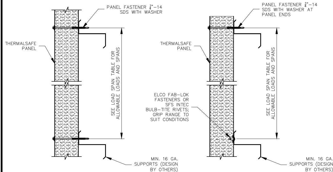
SECTION VIEW FASTENER PATTERNS: TSFP1, TSFP2, OR TSFPMAX
