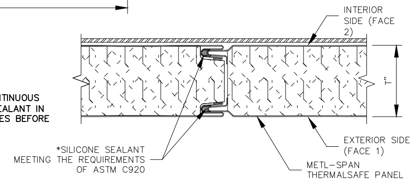
DETAIL 1 SEALANT REQUIREMENTS
