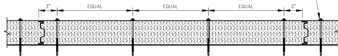
PANEL INSTALLATION SECTION AT END SUPPORTS-TSFP2
