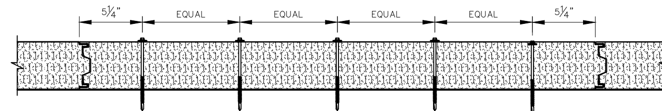
PANEL INSTALLATION SECTION AT INTERIOR SUPPORTS-TSFPMAX
