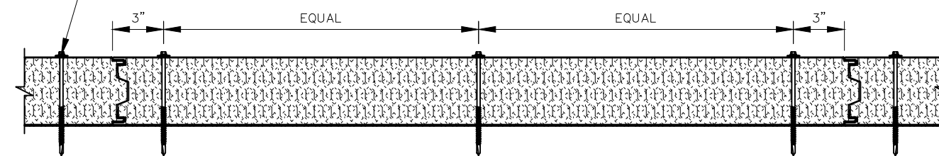
PANEL INSTALLATION SECTION AT END SUPPORTS-TSFP3
