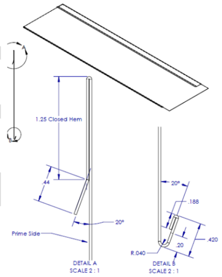
Figure 3B: View of 26 ga. Locking Mechanism
