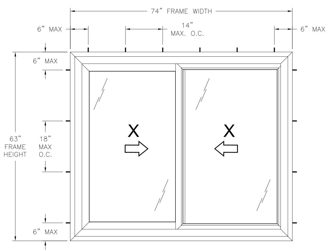
650 HS HORIZONTAL SLIDING WINDOW EXTERIOR VIEW FINLESS AND FLANGE INSTALLATION
