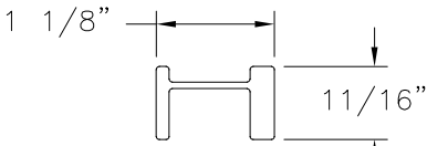
REINFORCEMENT (10300266) ALUMINUM 6005-T5
