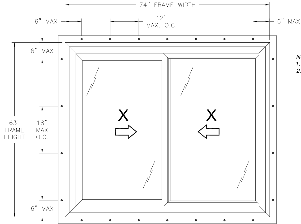
650 HS HORIZONTAL SLIDING WINDOW EXTERIOR VIEW FIN INSTALLATION
