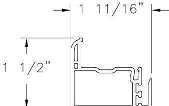
KEEPER RAIL (10005543) EXTRUDED VINYL
