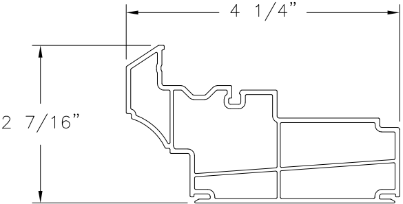
MAIN FRAME (6992) EXTRUDED VINYL
