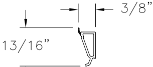
GLAZING BEAD (6998) EXTRUDED VINYL
