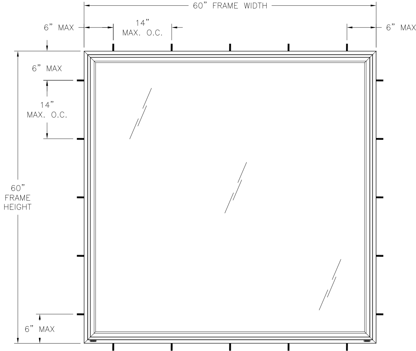
400 PW PICTURE WINDOW EXTERIOR VIEW
