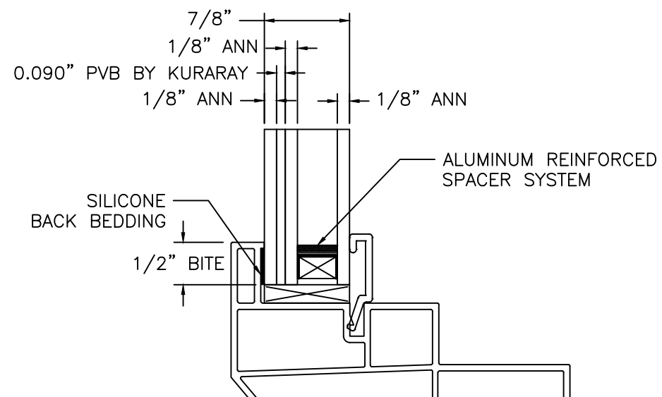
GLAZING DETAIL
