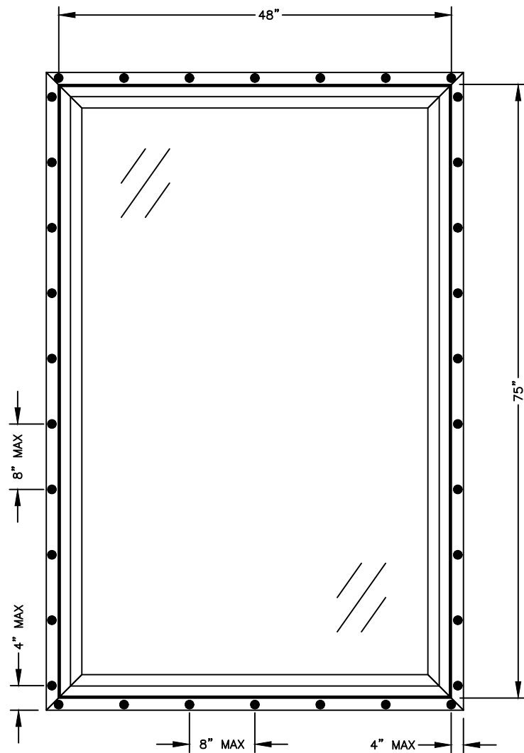
1650PWI PICTURE WINDOW – FIN INSTALLATION MAXIMUM SIZE 48" X 75" DESIGN PRESSURE +/- 50 PSF MISSILE D – WIND ZONE 3
