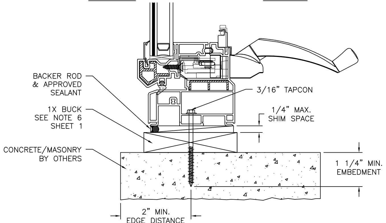
VERTICAL CROSS SECTION CONCRETE/MASONRY WITH 1X BUCK INSTALLATION FOR CONCRETE/MASONRY INSTALLATION WITHOUT 1X BUCK REFER TO JAMB INSTALLATION DETAILS
