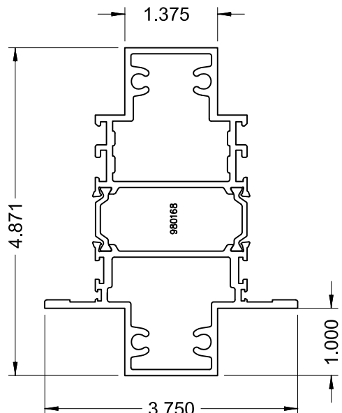
SERIES 4250i-OS ALT. MULLION
