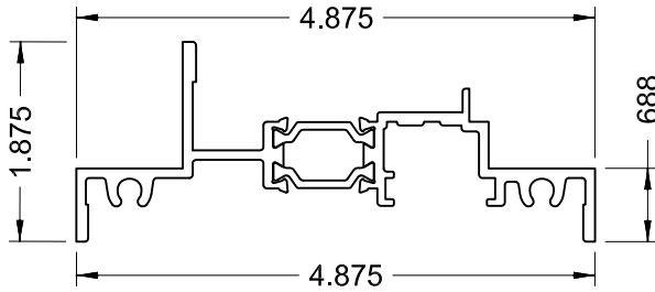
55 SERIES 4250i-OS FRAME HEAD/SILL/JAMB
