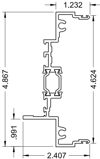
7.1A SERIES 4250i ALT. MALE MULLION
