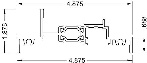
55 SERIES 4250i-OS FRAME HEAD/SILL/JAMB
