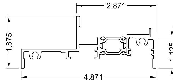
57 SERIES 4250i-SDH FRAME SILL
