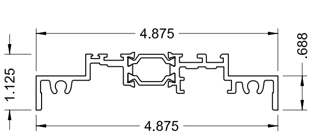
2.1 SERIES 4250i-OS FRAME HEAD/SILL/JAMB
