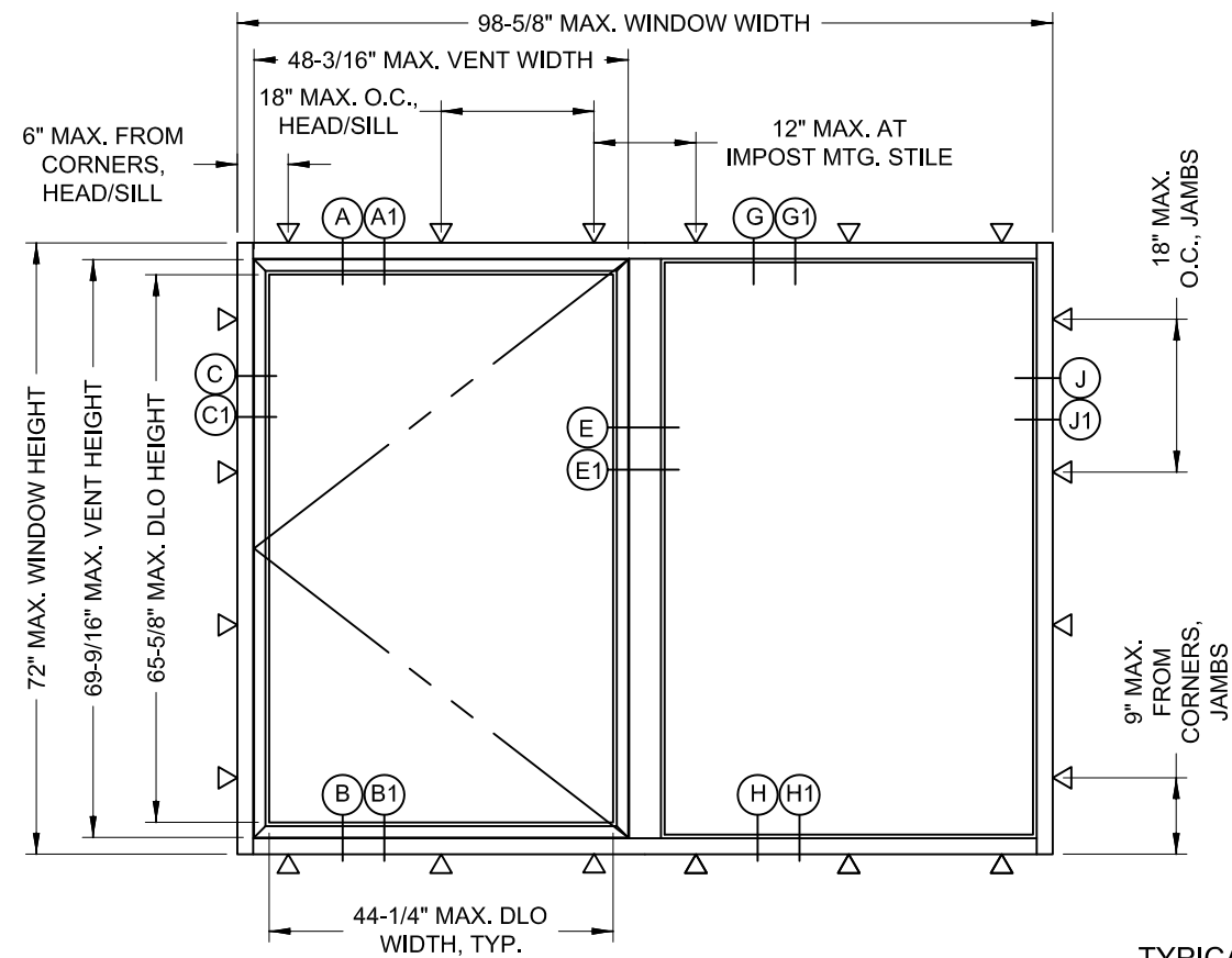
TYPICAL ELEVATIONS
