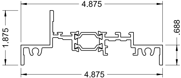
2.1A SERIES 4250i-OS ALT. FRAME HEAD/SILL/JAMB
