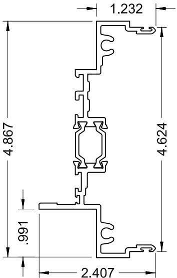
7.1A SERIES 4250i ALT. MALE MULLION
