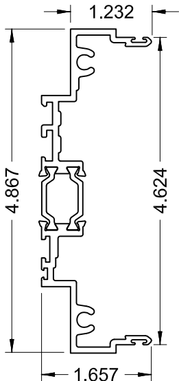
SERIES 4250i MALE MULLION 7.1
