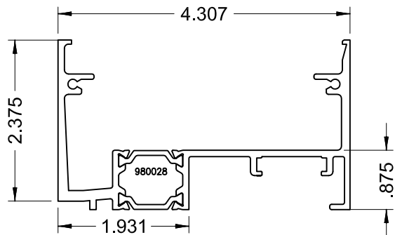
SERIES 3250i RECEPTOR SILL (LEVEL'D' IMPACT) NOT APPR'D FOR WATER RESISTANCE
