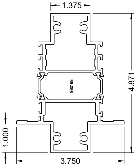
SERIES 4250i ALT. MULLION
