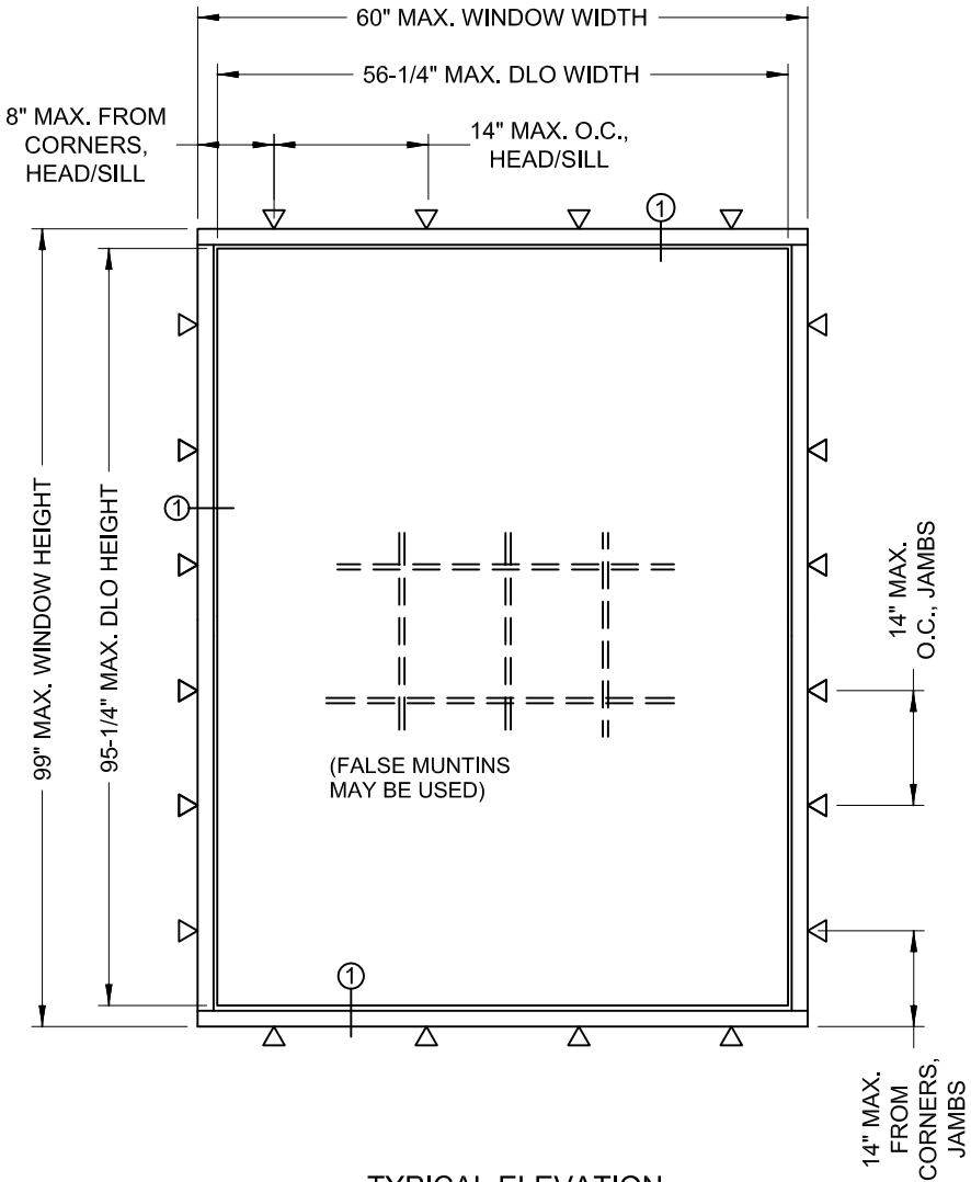
TYPICAL ELEVATION
