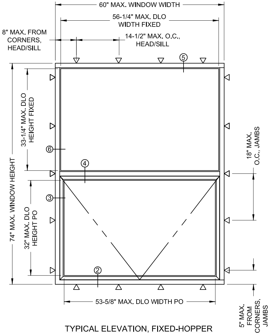
TYPICAL ELEVATION, FIXED-HOPPER
