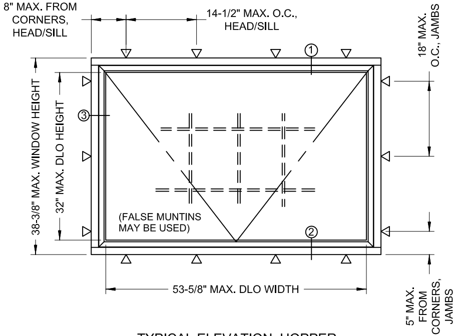
TYPICAL ELEVATION, HOPPER
