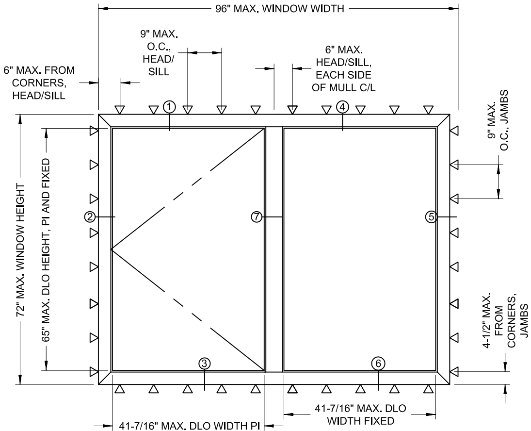
TYPICAL ELEVATION, CASEMENT-FIXED
