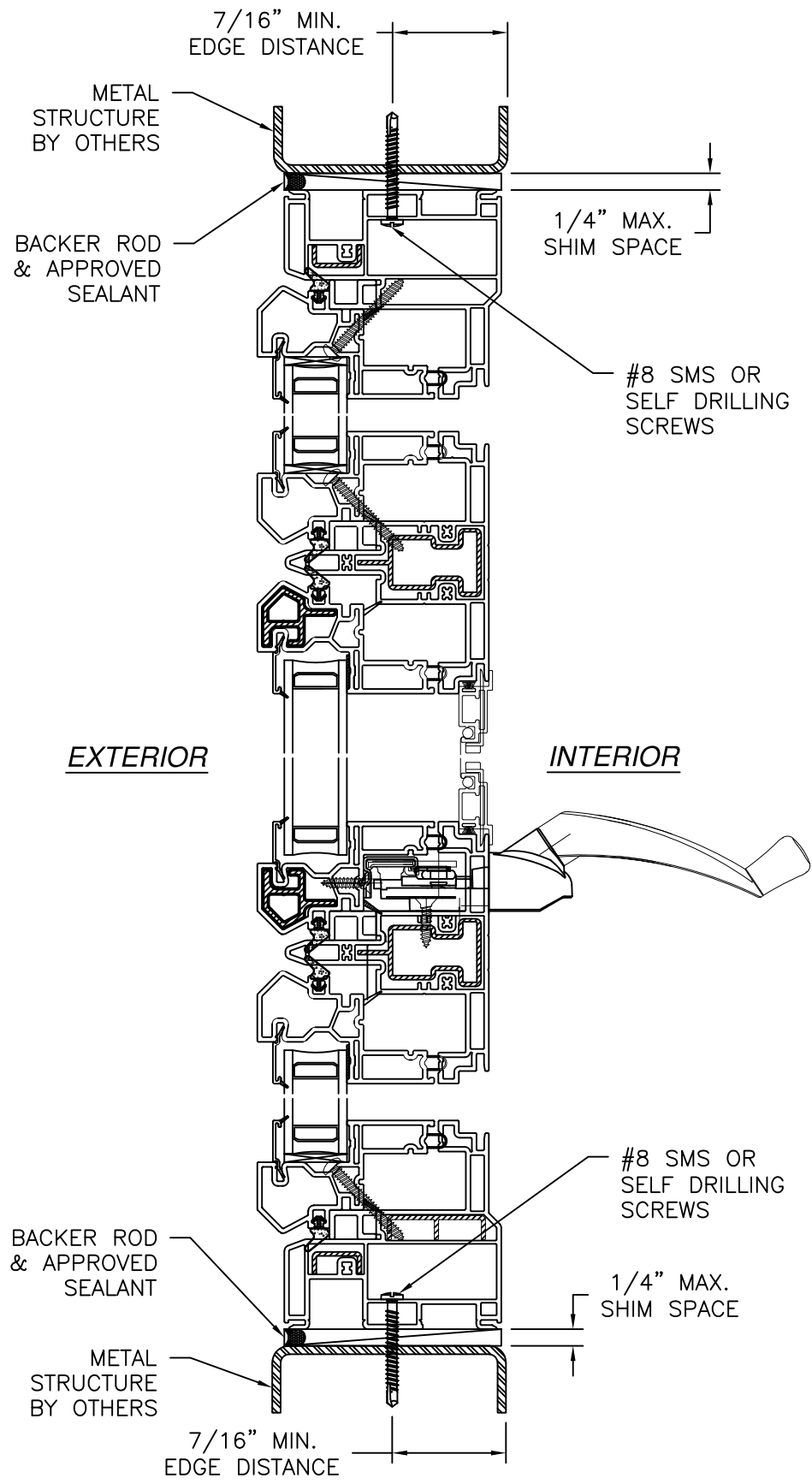
VERTICAL CROSS SECTION METAL STRUCTURE INSTALLATION
