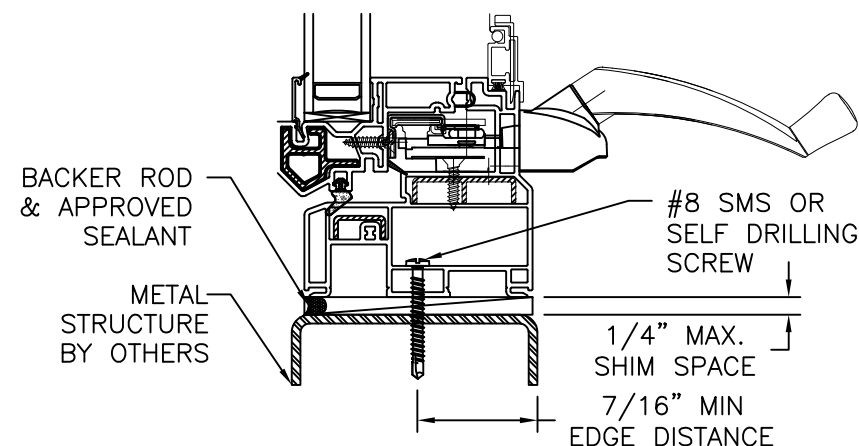
VERTICAL CROSS SECTION METAL STRUCTURE INSTALLATION
