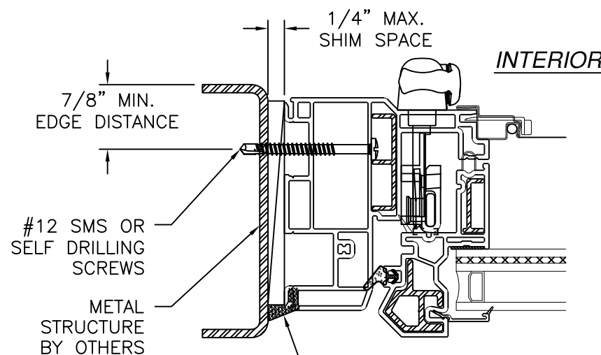
JAMB INSTALLATION DETAIL METAL STRUCTURE INSTALLATION
