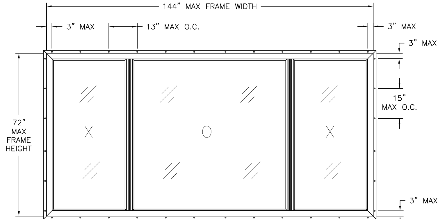
CAMBRIDGE CX/CXPX/CX MULLED CASEMENT COMBINATION ASSEMBLY EXTERIOR VIEW FIN INSTALLATION
