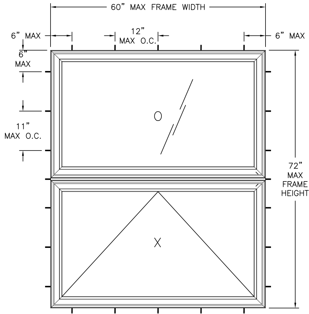
SIGN/CAMB IMP AWNING/FIXED STACKED ASSEMBLY EXTERIOR VIEW FRAME FLUSH INSTALLATION
