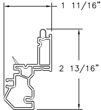
Sash VINYL PVC .070 THICK
