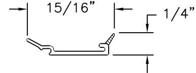
Glazing Bead VINYL PVC .040 THICK
