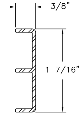
Under Operator Reinforcement Aluminum 6105 T5 .060 THICK
