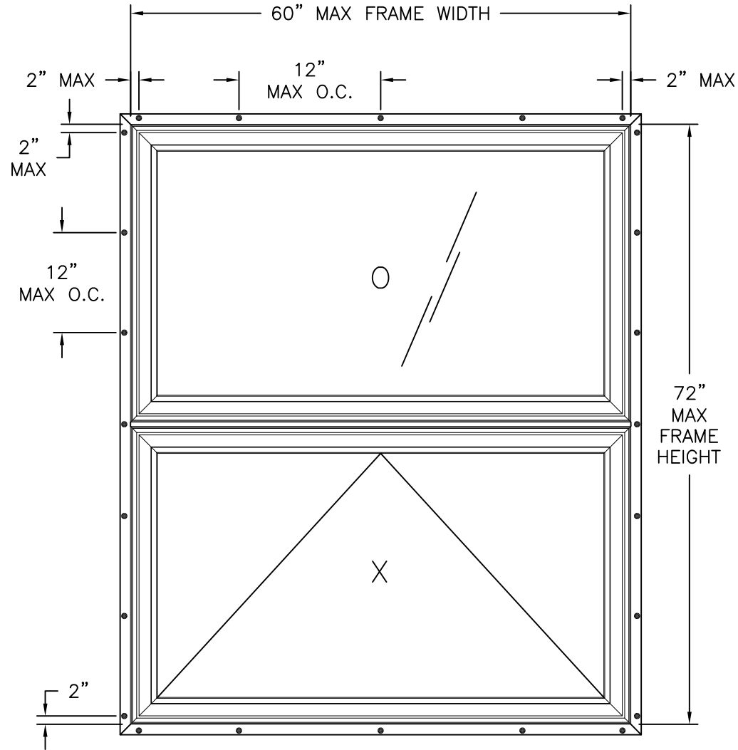
SIGN/CAMB IMP AWNING/FIXED STACKED ASSEMBLY EXTERIOR VIEW FIN INSTALLATION
