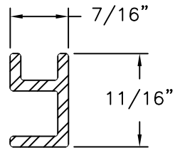
Spacer VINYL PVC .080 THICK
