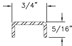
Under Hinge Reinforcement Aluminum 6105 T5, Anodized .060 THICK
