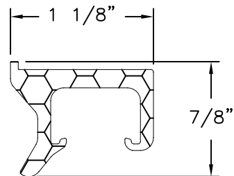
Snubber - Frame Aluminum 6105 T5, Anodized .100 THICK
