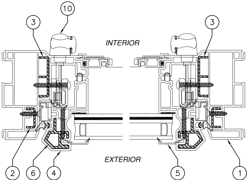
HORIZONTAL SECTION
