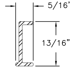
Sash Reinforcement Aluminum 6105 T5, Anodized .060 THICK
