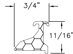
Snubber - Sash Aluminum 6105 T5 .092 THICK
