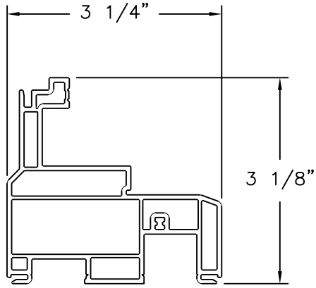
Frame VINYL PVC .070 THICK
