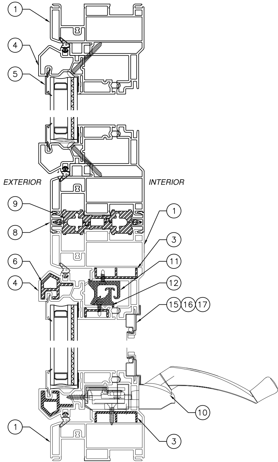
VERTICAL SECTION
