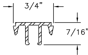
Astragal Reinforcement Aluminum 6105 T5 .060 THICK
