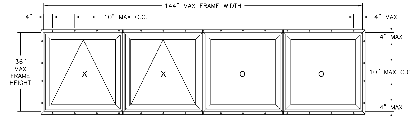
OCEANVIEW IMPACT AW/FIX MULLED ASSEMBLY EXTERIOR VIEW FIN INSTALLATION
