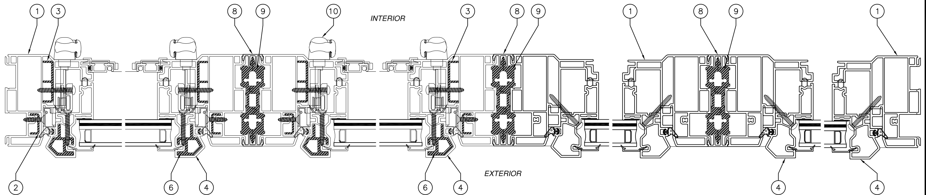
HORIZONTAL SECTION
