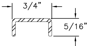
Under Hinge Reinforcement Aluminum 6105 T5, Anodized .060 THICK
