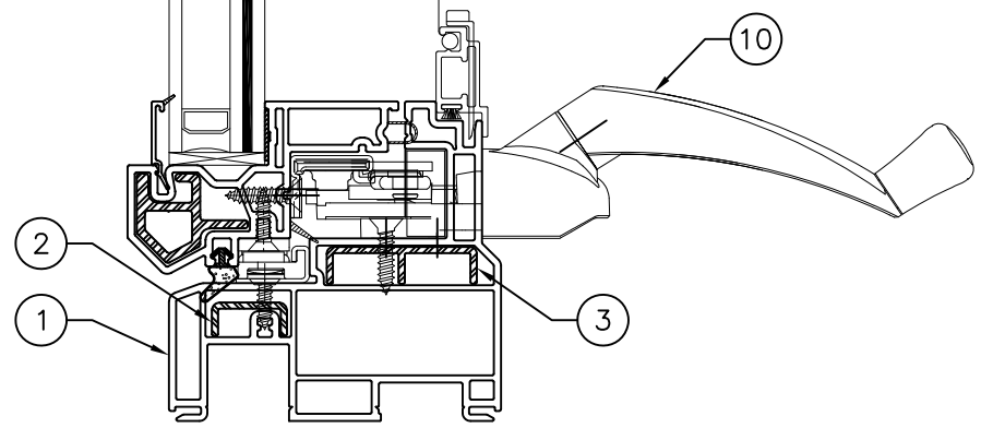
VERTICAL SECTION
