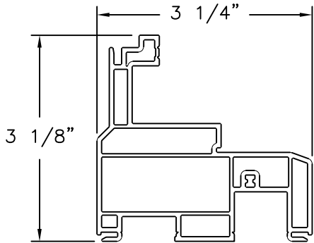
Frame VINYL PVC .070 THICK
