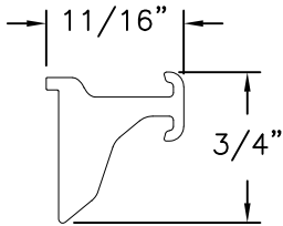
Snubber - Sash Aluminum 6105 T5 .092 THICK
