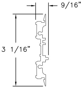
Mullion Reinforcement Aluminum 6105 T5 .090 THICK
