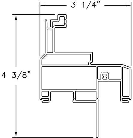
Frame (with Nail Fin) VINYL PVC .070 THICK
