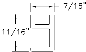
Spacer VINYL PVC .080 THICK
