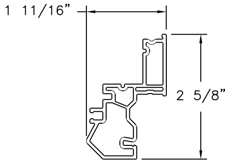
Sash VINYL PVC .070 THICK
