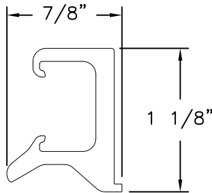
Snubber - Frame Aluminum 6105 T5, Anodized .100 THICK
