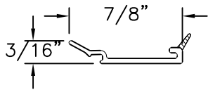
Glazing Bead VINYL PVC .040 THICK
