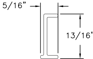
Sash Reinforcement Aluminum 6105 T5, Anodized .060 THICK
