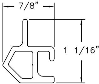
Sash Reinforcement Aluminum 6105 T5, Anodized .078 THICK
