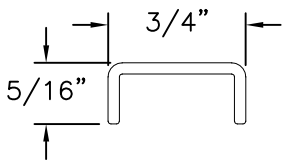
Under Hinge Reinforcement Aluminum 6105 T5, Anodized .060 THICK
