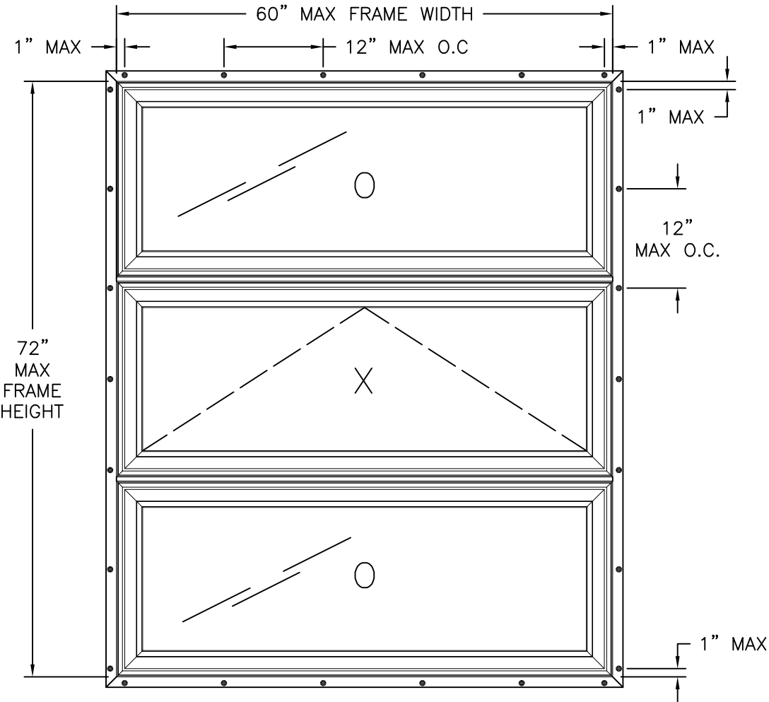
SIGN/COMB IMP AW/FIX TRIPLE STACKED MULLED ASSEMBLY EXTERIOR VIEW FIN INSTALLATION
