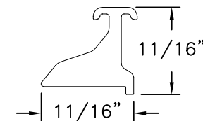
Snubber - Sash Aluminum 6105 T5 .092 THICK
