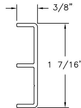
Under Operator Reinforcement Aluminum 6105 T5 .060 THICK
