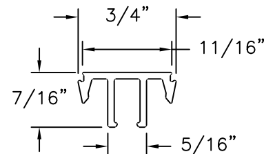
Astragal Reinforcement Aluminum 6105 T5 .060 THICK
