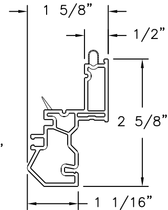
Sash VINYL PVC .070 THICK
