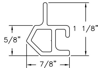
Sash Reinforcement Aluminum 6105 T5, Anodized .078 THICK
