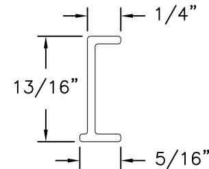
Sash Reinforcement Aluminum 6105 T5, Anodized .060 THICK
