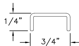
Under Hinge Reinforcement Aluminum 6105 T5, Anodized .060 THICK
