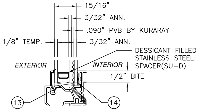
GLAZING DETAIL
