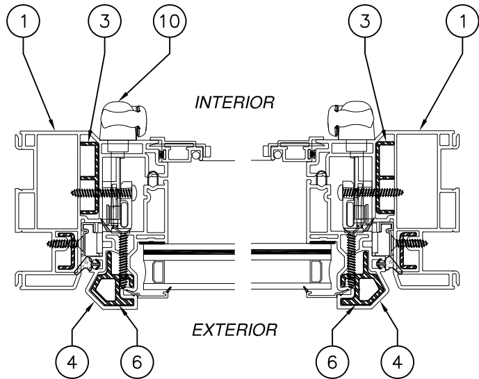
HORIZONTAL SECTION
