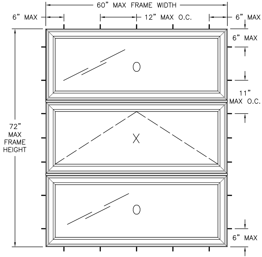
SIGN/COMB IMP AW/FIX TRIPLE STACKED MULLED ASSEMBLY EXTERIOR VIEW FRAME FLUSH INSTALLATION
