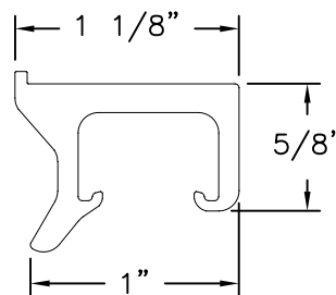
Snubber - Frame Aluminum 6105 T5, Anodized .100 THICK
