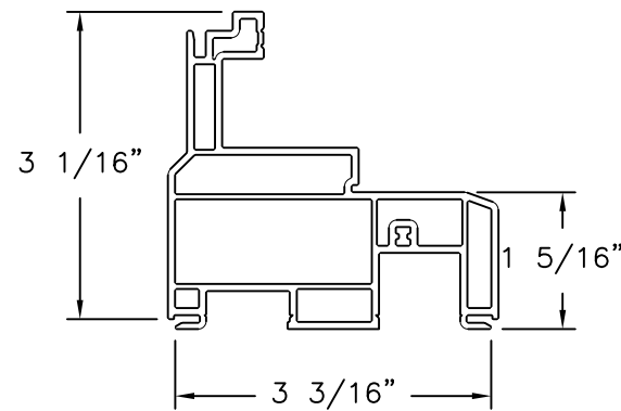
Frame VINYL PVC .070 THICK
