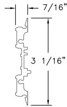
Astragal Reinforcement Aluminum 6105 T5 .060 THICK
