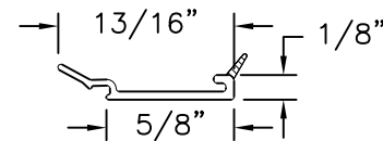
Glazing Bead VINYL PVC .040 THICK
