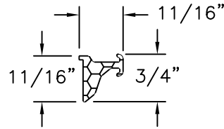
Snubber - Sash Aluminum 6105 T5 .092 THICK
