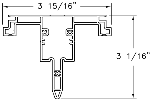
Astragal Frame VINYL PVC .070 THICK
