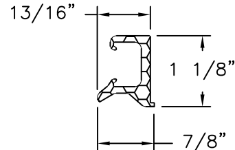
Snubber - Frame Aluminum 6105 T5, Anodized .100 THICK
