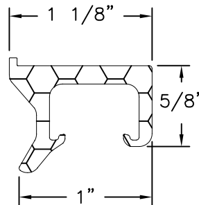
Snubber - Frame Aluminum 6105 T5, Anodized .100 THICK
