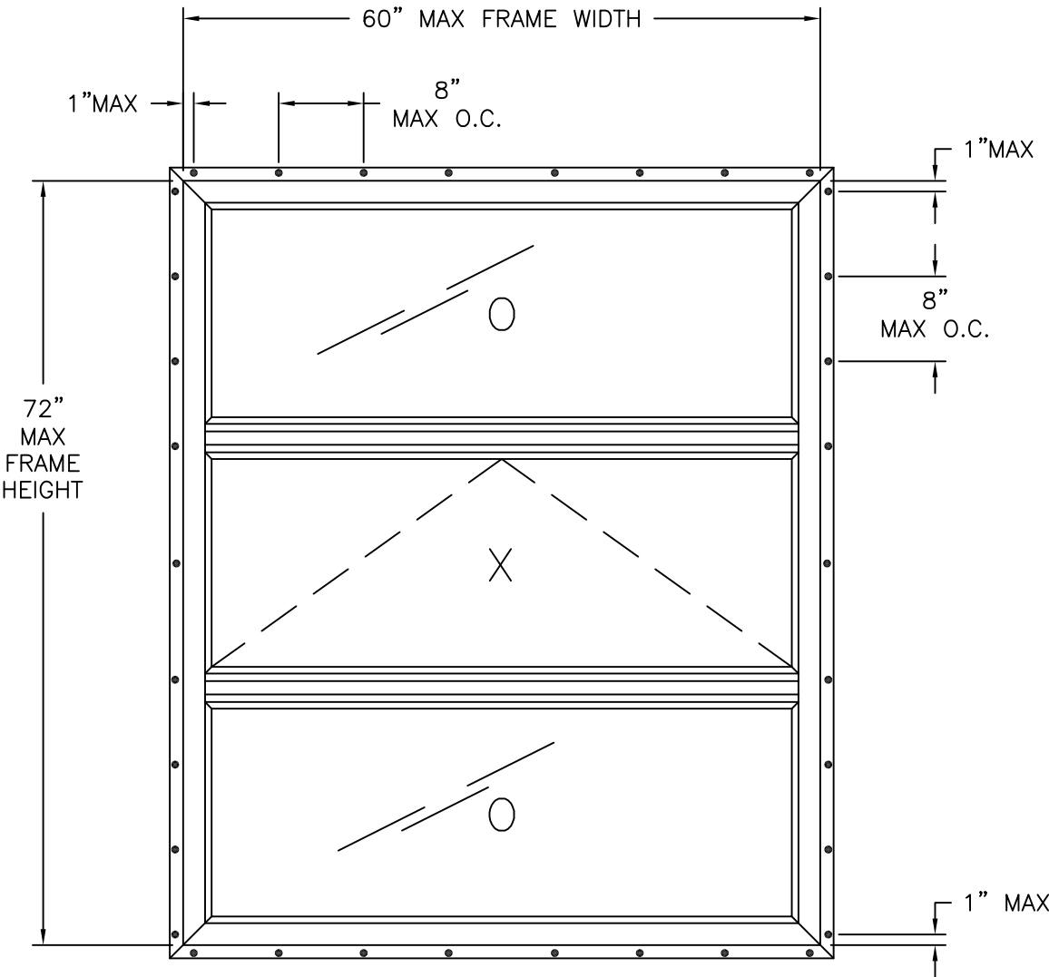
S-SERIES IMPACT AW/ FIX STACKED COMBINATION ASSEMBLY EXTERIOR VIEW FIN INSTALLATION
