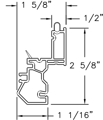
Sash VINYL PVC .070 THICK
