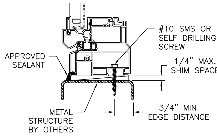
VERTICAL CROSS SECTION METAL STRUCTURE INSTALLATION
