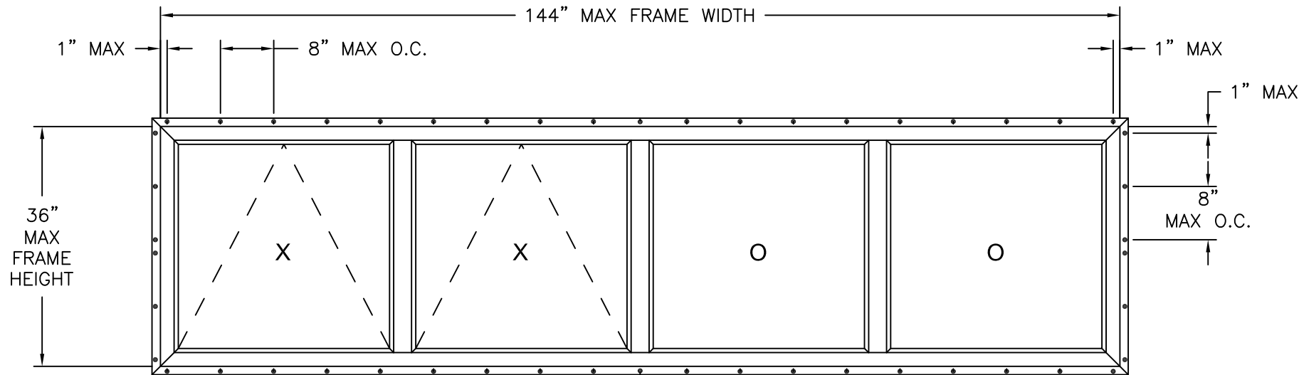
OCEANVIEW IMPACT AWNING/FIXED COMBINATION ASSEMBLY EXTERIOR VIEW FIN INSTALLATION
