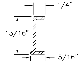
Sash Reinforcement Aluminum 6105 T5, Anodized .060 THICK
