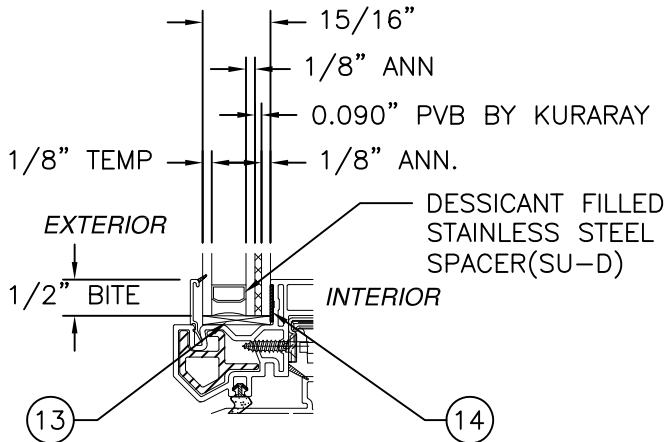
GLAZING DETAIL
