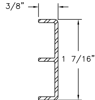
Under Operator Reinforcement Aluminum 6105 T5 .060 THICK
