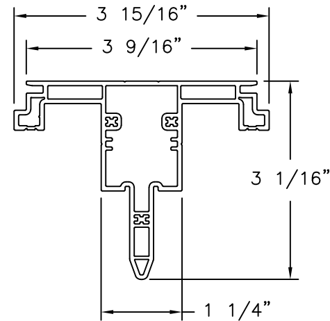
Astragal Frame VINYL PVC .070 THICK
