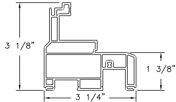
Frame VINYL PVC .070 THICK
