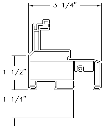
Frame (with Nail Fin) VINYL PVC .070 THICK
