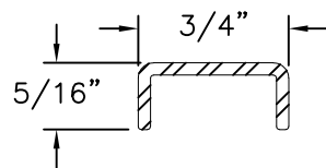
Under Hinge Reinforcement Aluminum 6105 T5, Anodized .060 THICK
