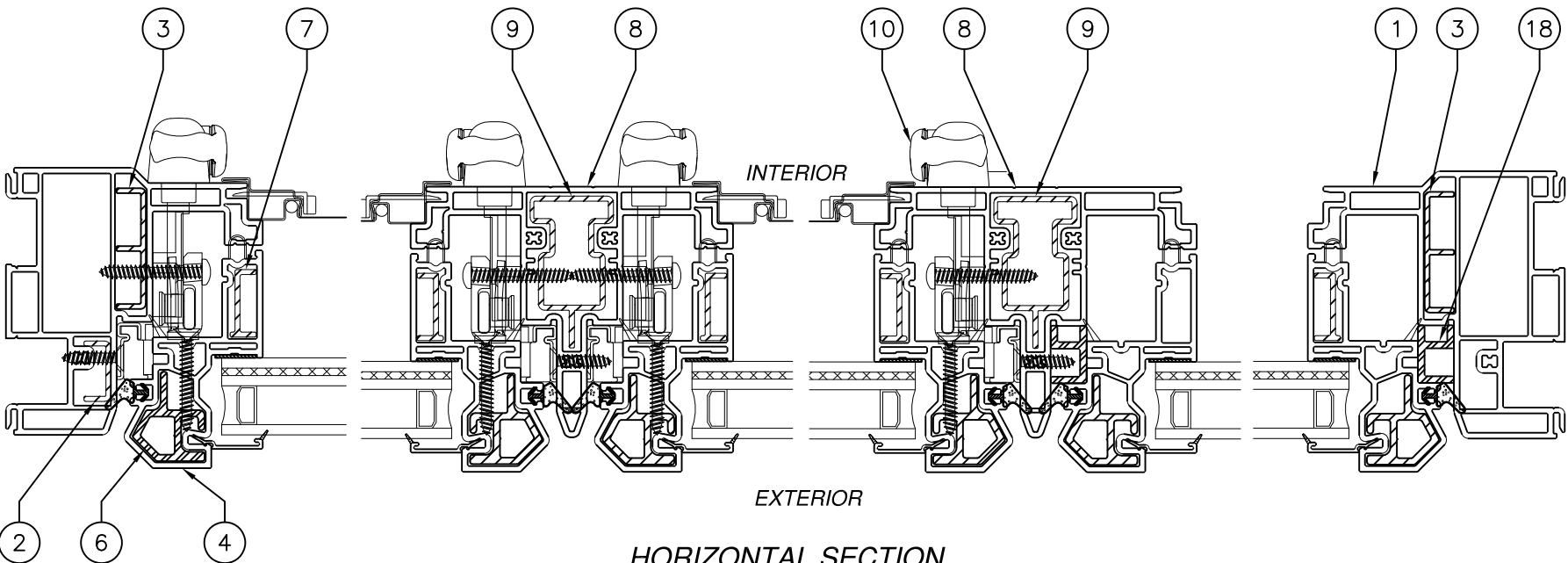
HORIZONTAL SECTION
