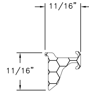
Snubber - Sash Aluminum 6105 T5 .092 THICK
