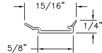
Glazing Bead VINYL PVC .040 THICK
