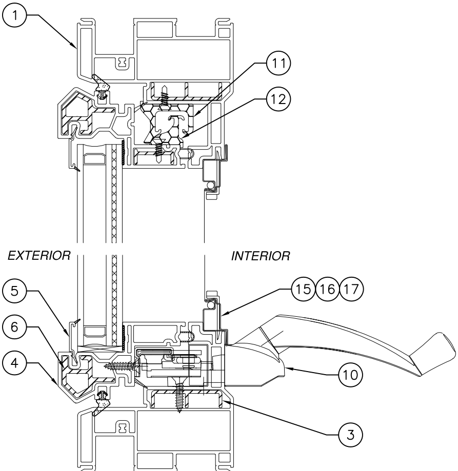
VERTICAL SECTION
