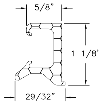
Snubber - Frame Aluminum 6105 T5, Anodized .100 THICK
