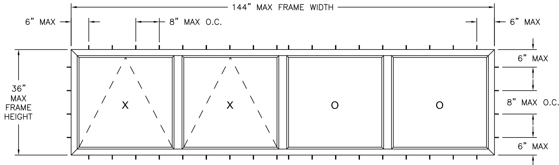
OCEANVIEW IMPACT AWNING/FIXED COMBINATION ASSEMBLY EXTERIOR VIEW FRAME FLUSH INSTALLATION
