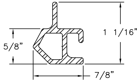
Sash Reinforcement Aluminum 6105 T5, Anodized .078 THICK
