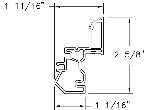
Sash VINYL PVC .070 THICK
