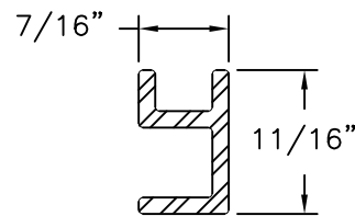
Spacer VINYL PVC .080 THICK
