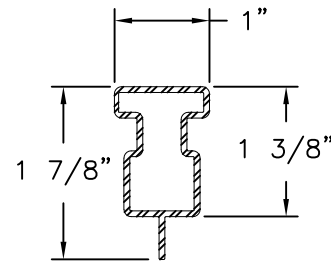
Astragal Reinforcement Aluminum 6105 T5 .060 THICK
