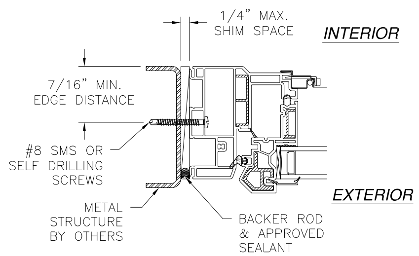
JAMB INSTALLATION DETAIL METAL STRUCTURE INSTALLATION
