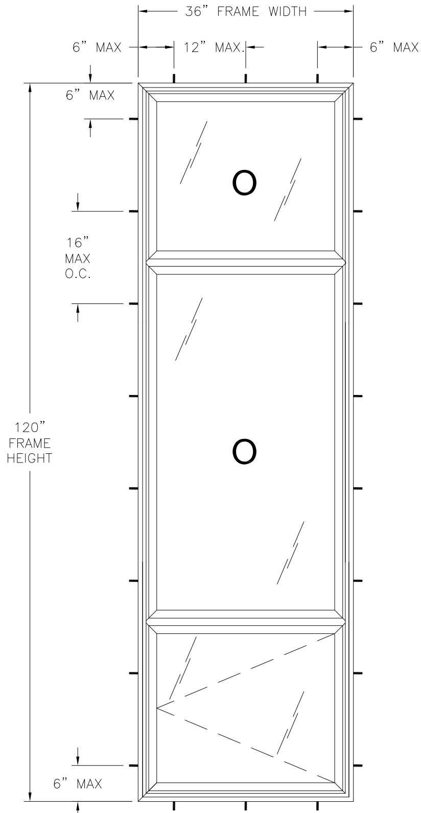
S-SERIES STACKED FIXED/FIXED/CASEMENT EXTERIOR VIEW FRAME INSTALLATION
