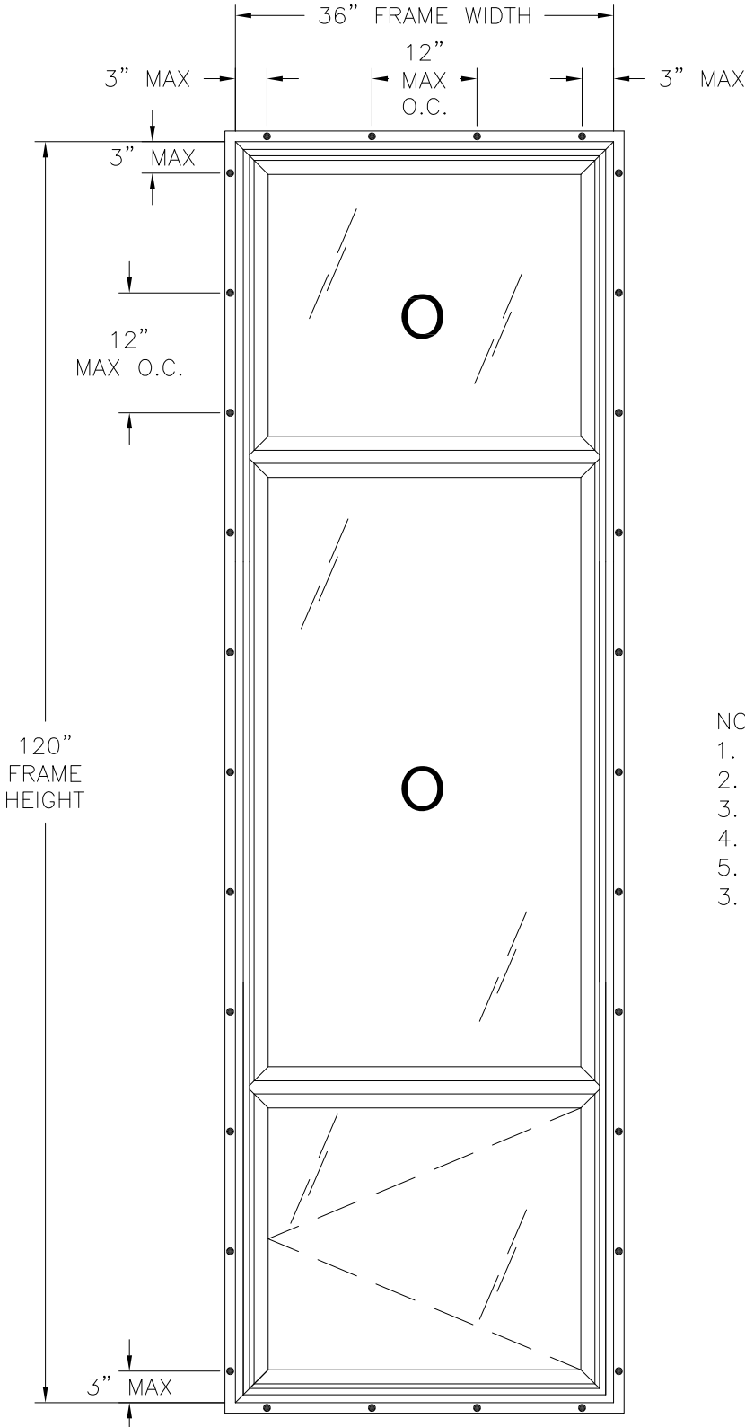
S-SERIES STACKED FIXED/FIXED/CASEMENT EXTERIOR VIEW FIN INSTALLATION
