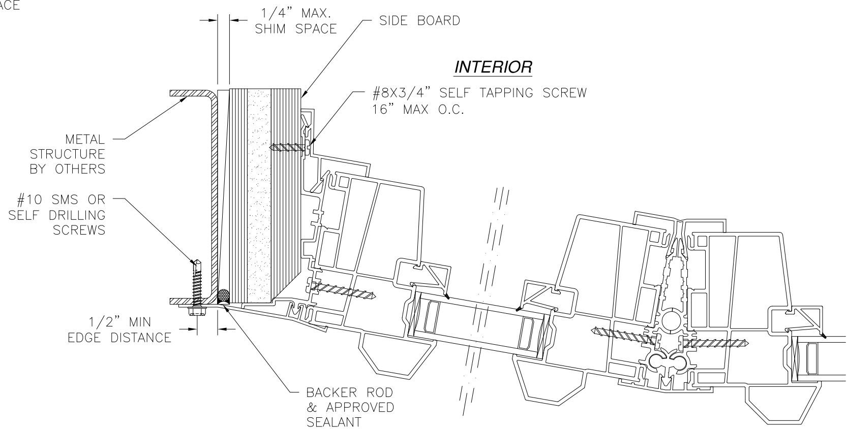
JAMB INSTALLATION DETAIL METAL STRUCTURE INSTALLATION
