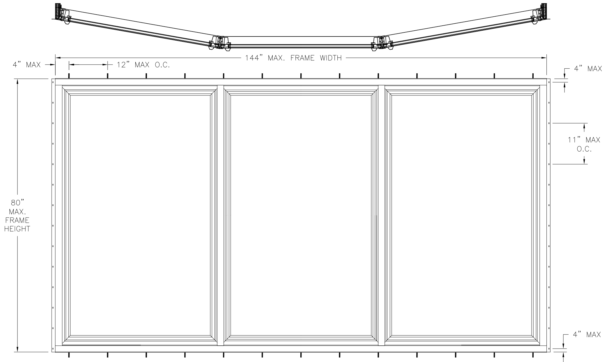
S-SERIES/CAMBRIDGE CXPX 10° EXTERIOR VIEW
