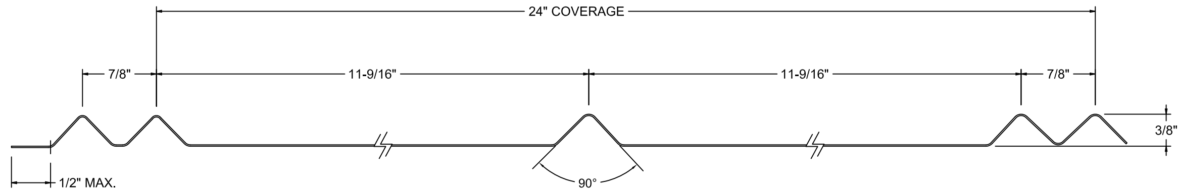
5V Crimp Profile
