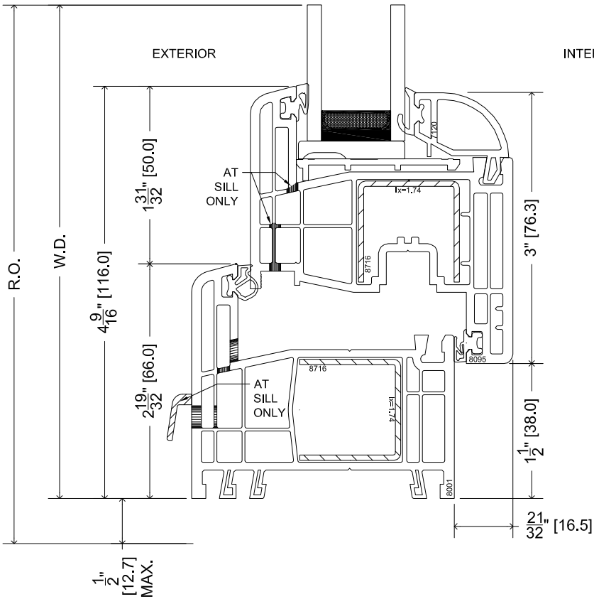
TYPICAL SECTION DETAIL HEAD/SILL/JAMB
