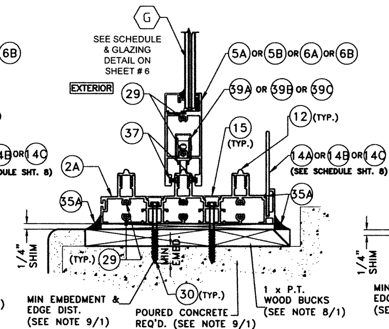
CONCRETE SUBSTRATE (3 TRACK SILL)
