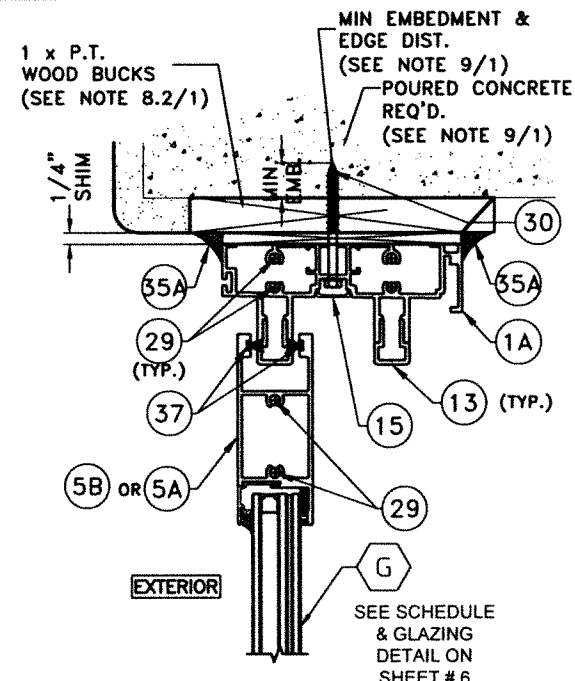
CONCRETE SUBSTRATE * (2 TRACK HEAD)
