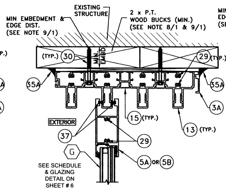
WOOD SUBSTRATE * (4 TRACK HEAD)
