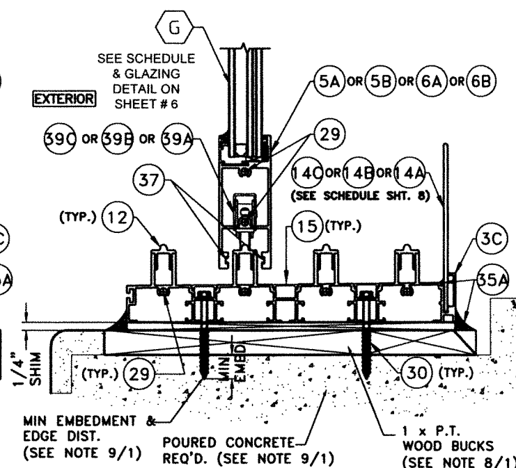
CONCRETE SUBSTRATE (4 TRACK SILL)
