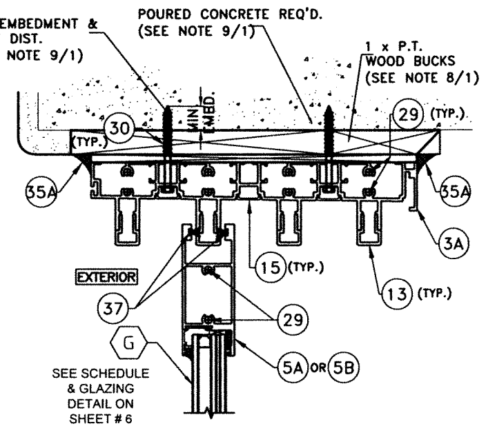
CONCRETE SUBSTRATE * (4 TRACK HEAD)
