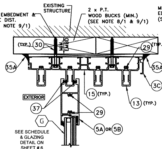
WOOD SUBSTRATE * (4 TRACK HEAD)
