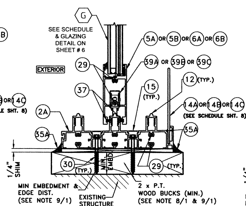
WOOD SUBSTRATE (3 TRACK SILL)
