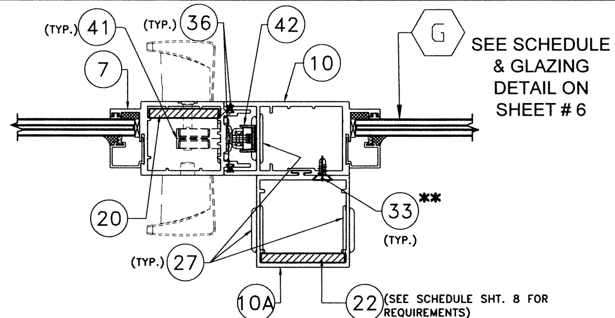
REINFORCED DEEP ASTRAGAL W/LAMINATED GLASS
