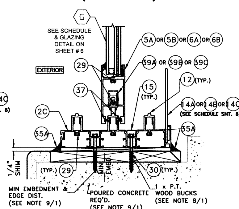
CONCRETE SUBSTRATE (3 TRACK SILL)
