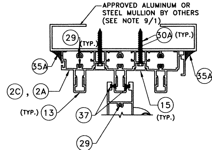
ALUMINUM & STEEL SUBSTRATE (3 TRACK HEAD)
