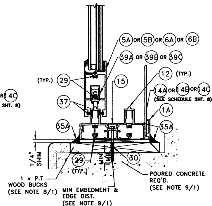
CONCRETE SUBSTRATE (2 TRACK SILL)
