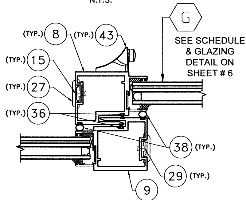
UNREINFORCED MEETING STILES W/INSULATED GLASS N.T.S.
