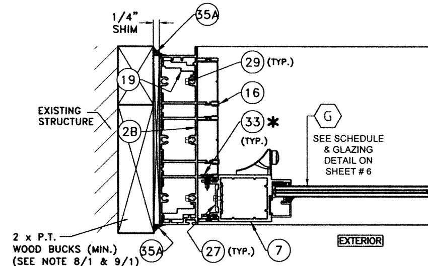
WOOD SUBSTRATE (3 TRACK REINFORCED JAMB)
