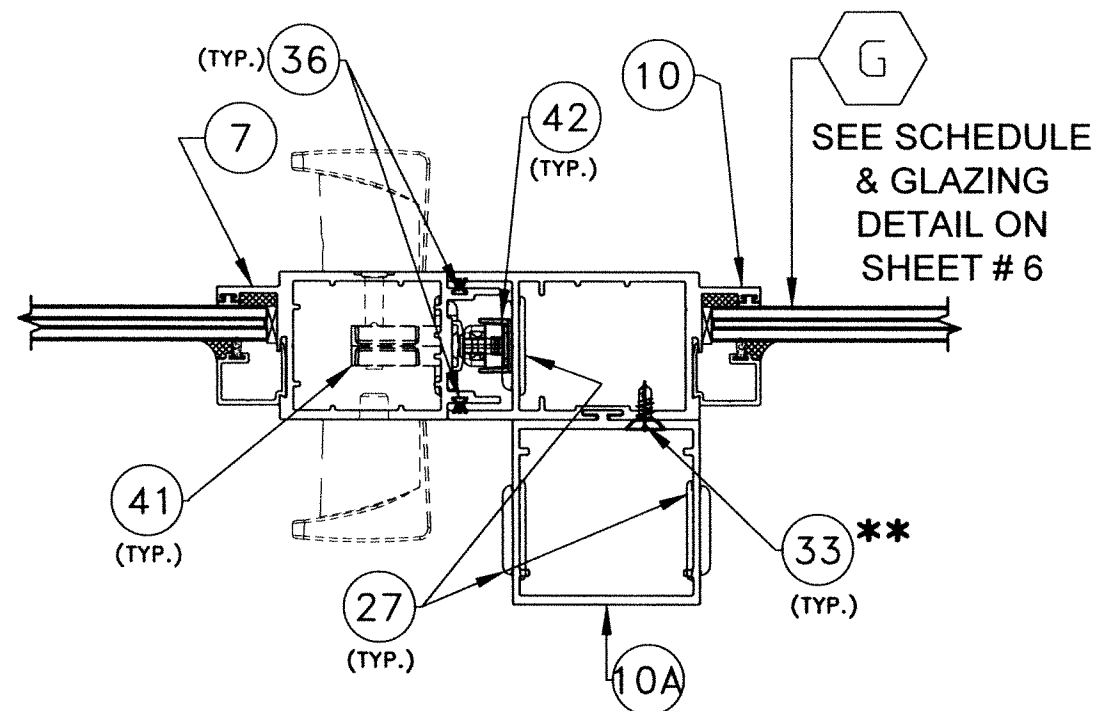
UNREINFORCED DEEP ASTRAGAL W/LAMINATED GLASS
