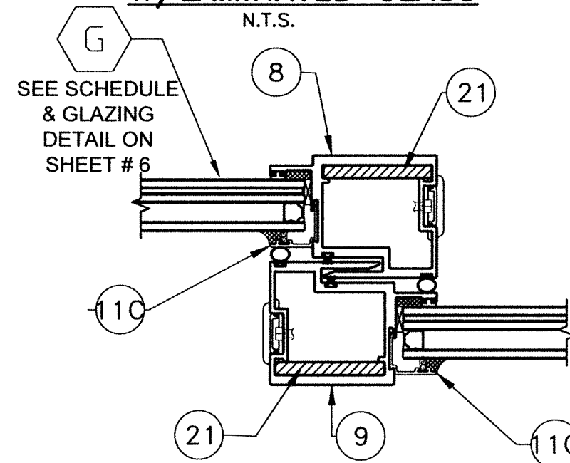
REINFORCED MEETING STILES W/INSULATED GLASS N.T.S.
