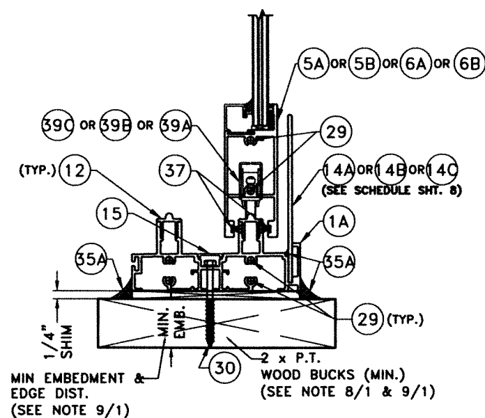
WOOD SUBSTRATE (2 TRACK SILL)
