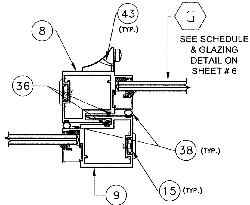
UNREINFORCED MEETING STILES W/LAMINATED GLASS N.T.S.
