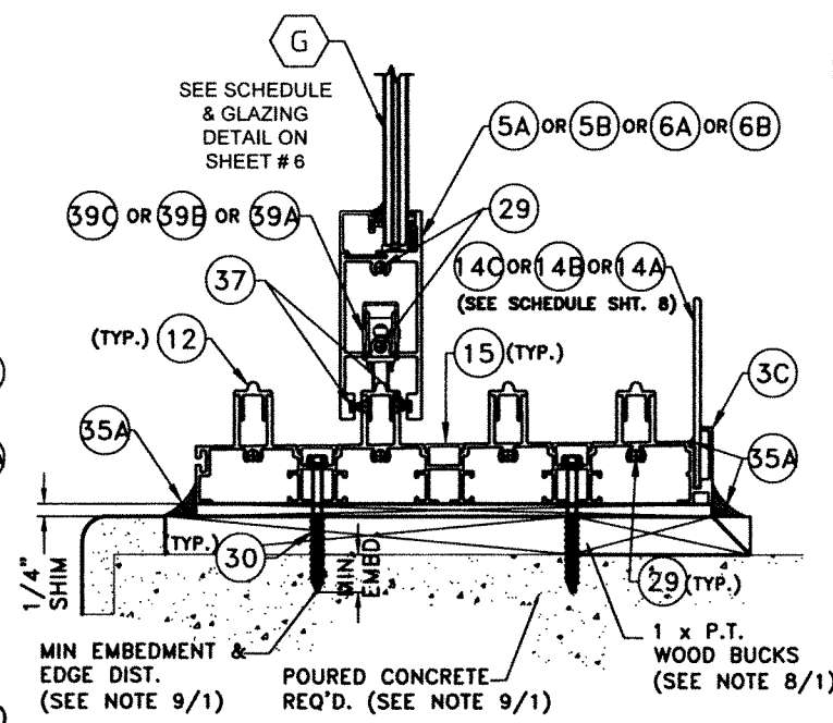
CONCRETE SUBSTRATE (4 TRACK SILL)
